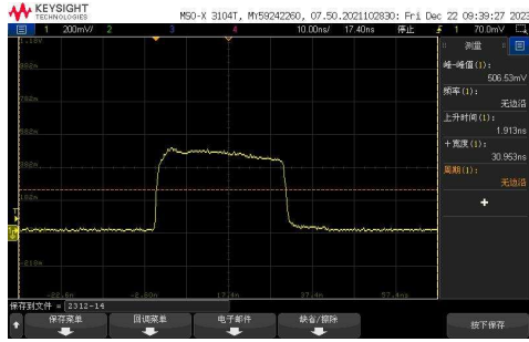
30ns/100kHz/0.3A
