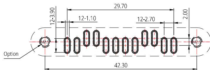
Recommended P.C.B layout (Top View) Tolerance \pm 0.05
