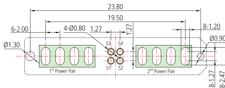
Recommended P.C.B Layout (Top View) Tolerance: \pm 0.05\text{mm}
