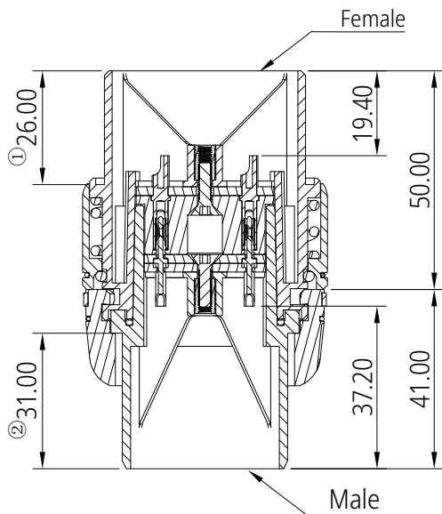
Mating View
