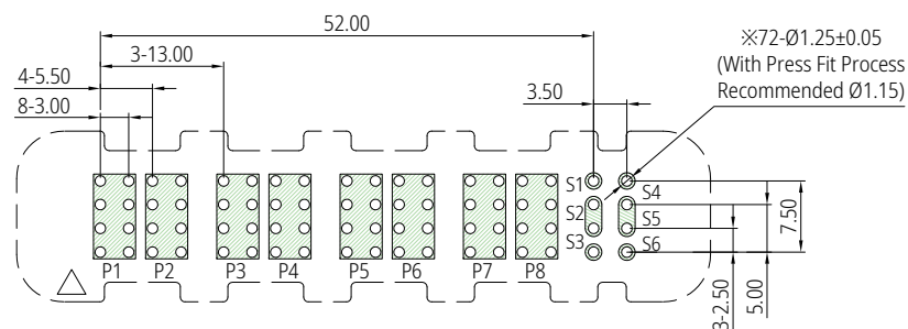
Recommended P.C.B layout (Top View) Tolerance \pm 0.05
