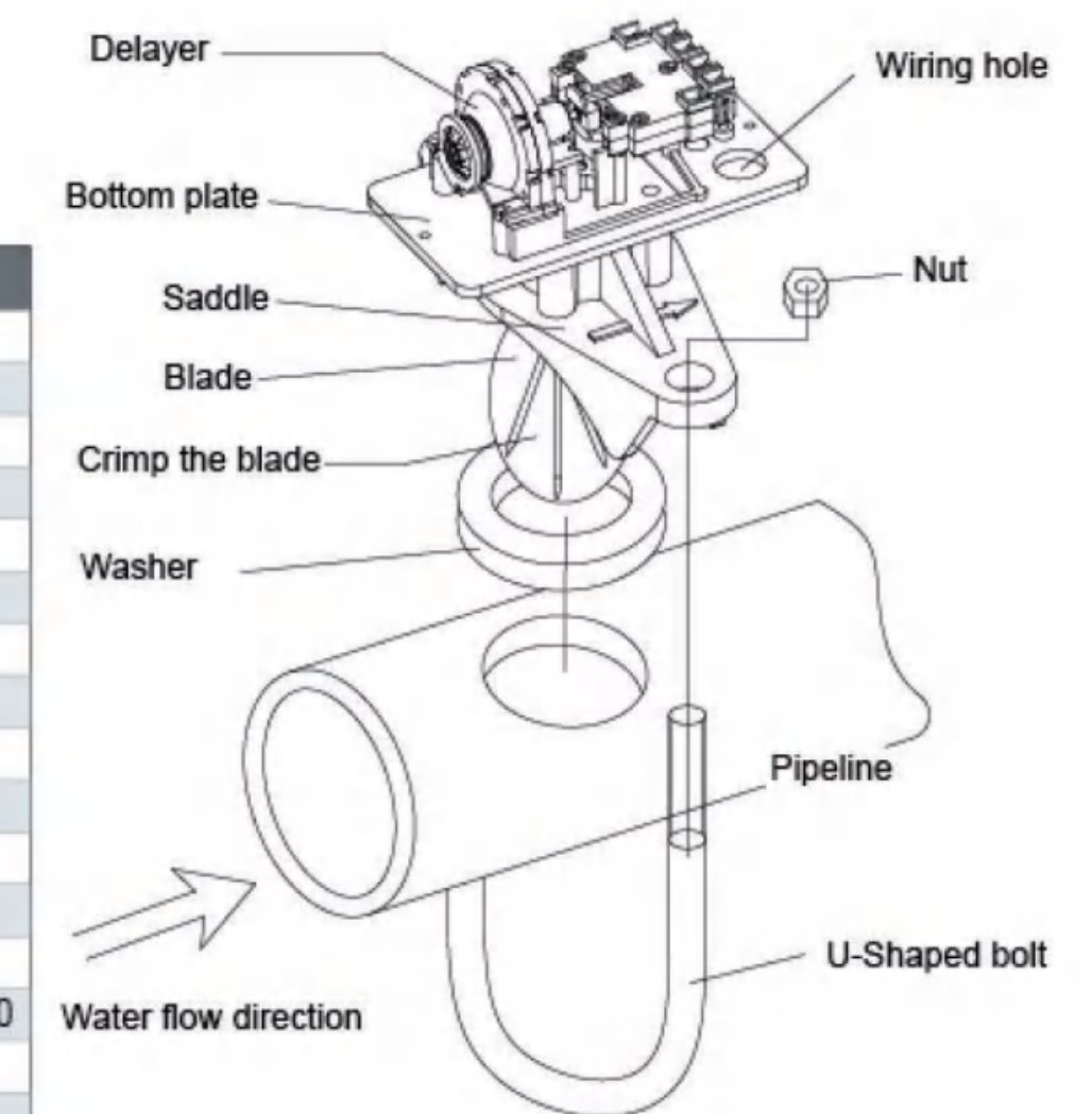
Figure 2 Installation Drawing
