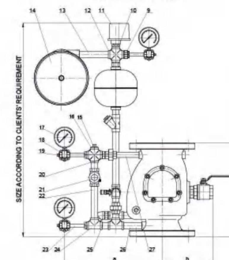
ASSEMBLY DRAWING WITHOUT COMPENSATOR SYSTEM
