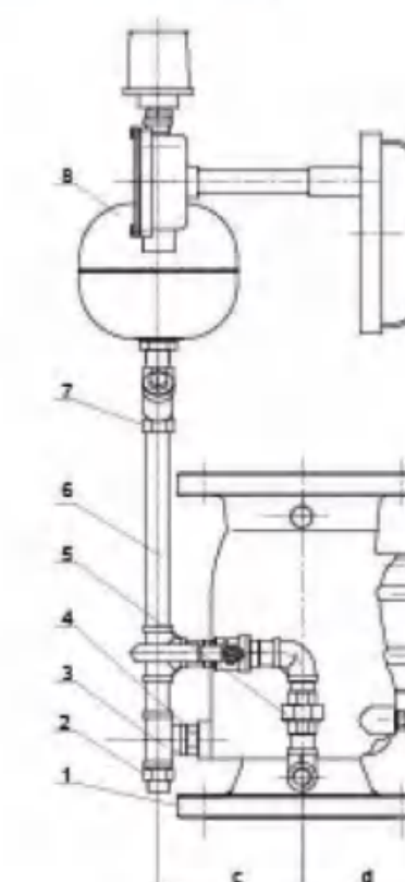
ASSEMBLY DRAWING WITHOUT COMPENSATOR SYSTEM
