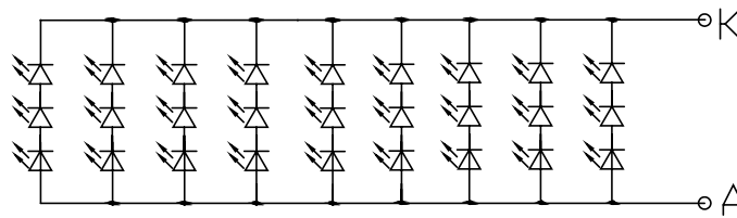
Electrial Circuit
