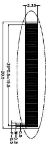
DETAIL A (4:1)
