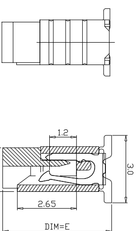
RECOMMENDED FCC/FPC DIM.
