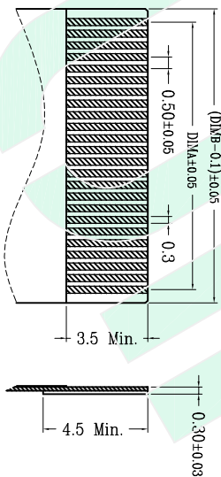
适用扁平线 (Applicable Flat Cable)
