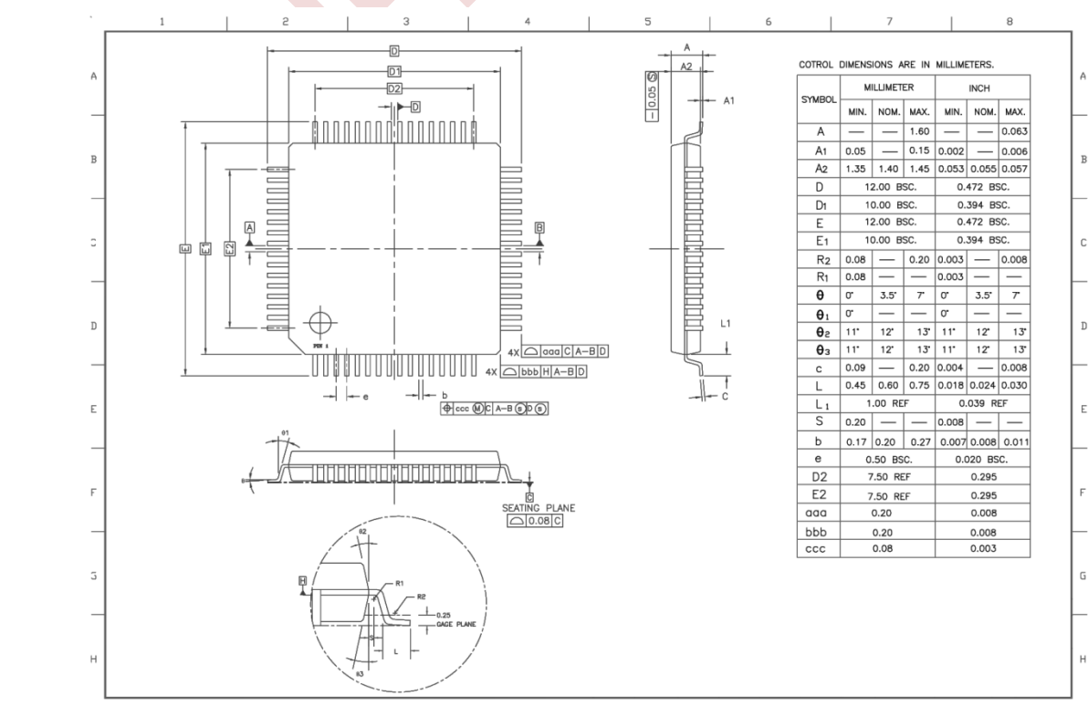
LQFP-64
