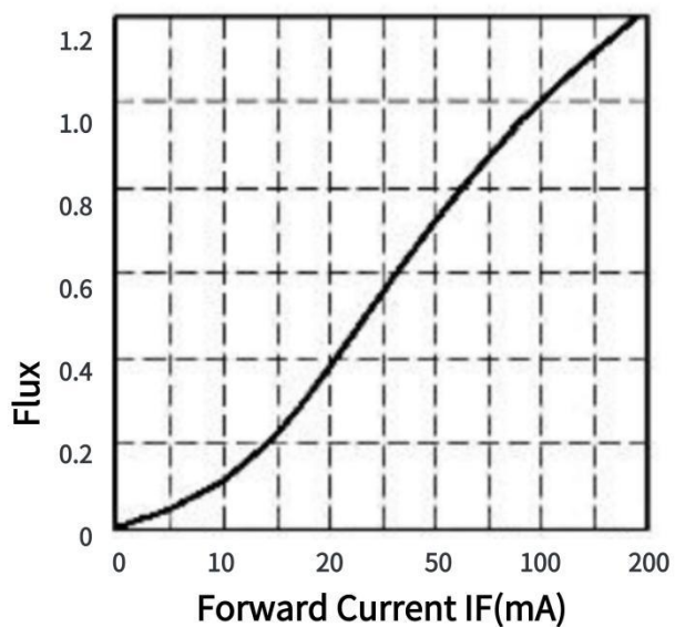
Flux vs. Forward Current
