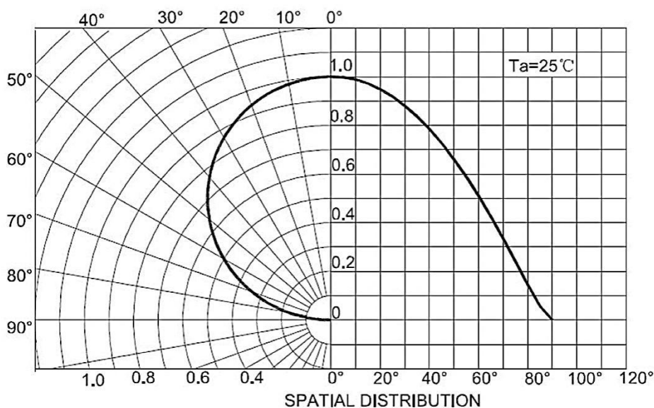
Radiation diagram
