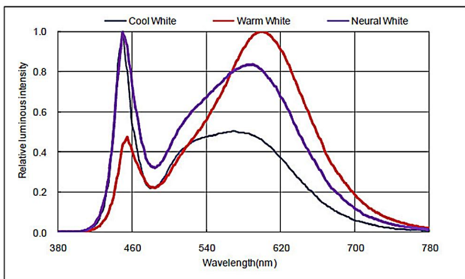
Relative spectral emission
