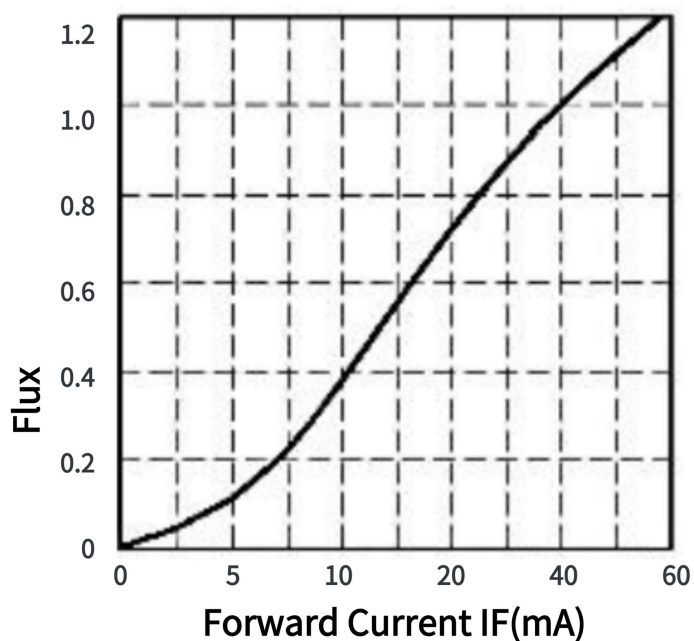
Flux vs. Forward Current
