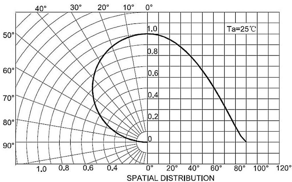
Radiation diagram
