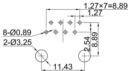
RECOMMENDED PCB LAYOUT (COMPONENT SIDE VIEW)
