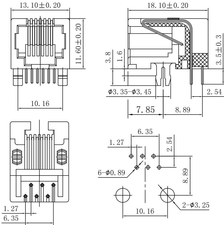
RECOMMENDED PCB LAYOUT (COMPONENT SIDE VIEW)
