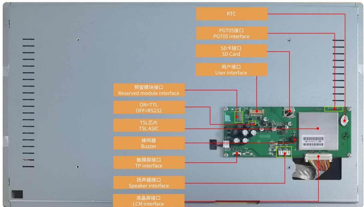
硬件接口图 Hardware interface
