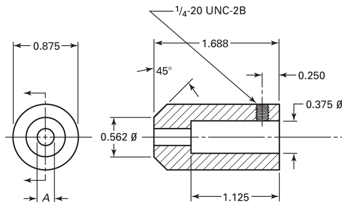
Gage Head
