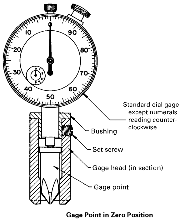
Fig. III-3 Penetration Gage for Type II Recess
