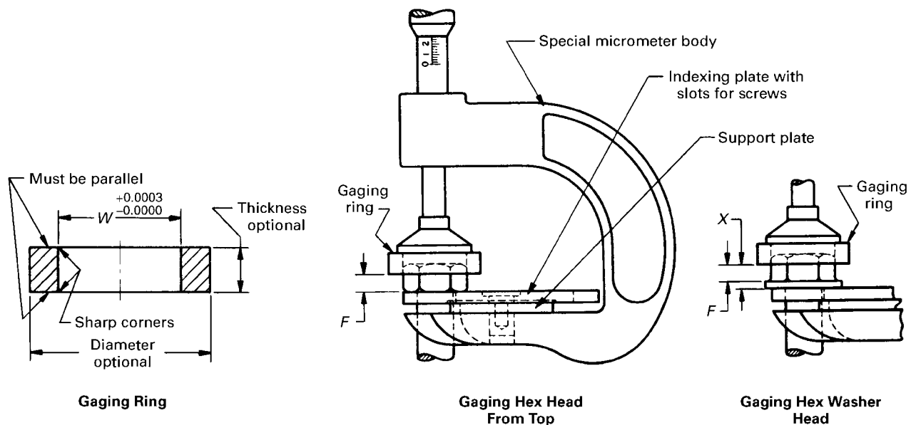
Fig. II-1 Typical Gaging Fixture
