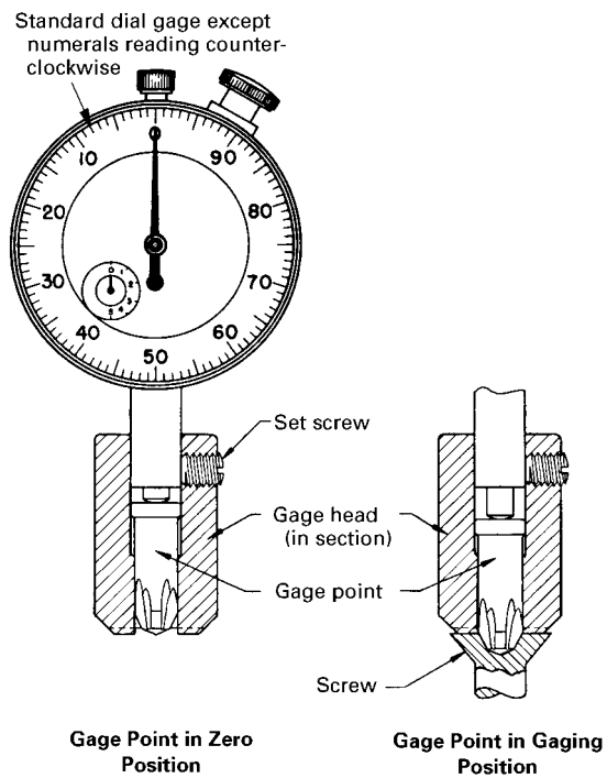
Fig. III-2 Penetration Gage for Type IA Recess
