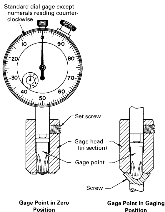
Fig. III-1 Penetration Gage for Type I Recess
