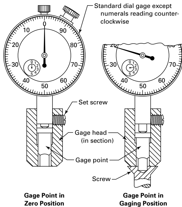
Fig. III-4 Penetration Gage for Type III Recess
