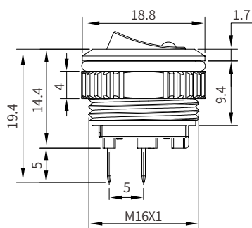
数控加工, 外观高档 CNC, High-grade
