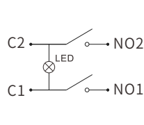
带灯 (2档/4脚) With LED (2rd gear/4-pin)
