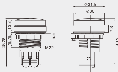
平头指示灯 Flat head indicator light
