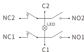
带灯 (2档/6脚) With LED (2rd gear/6-pin)
