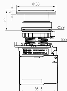
M4 Mushroom head button (red/green plastic head) M4蘑菇头按钮(红色/绿色塑料头部) LB22SA2M4-M ◆■/PC
