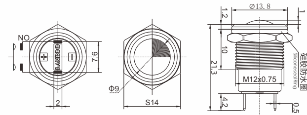
12B外形尺寸 Outline Dimension
