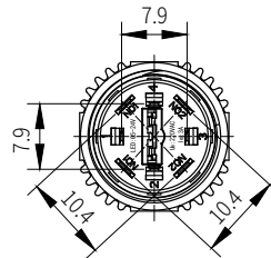
防水等级IP68 Waterproof grade IP68
