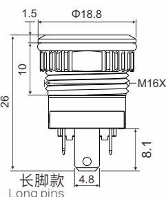
镀银长插脚 Silver Long Plated Pins
