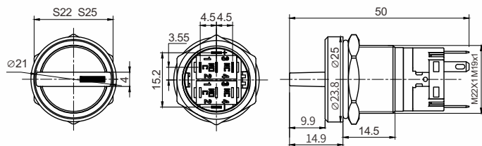
带灯,大旋柄 LED, Big Handle
