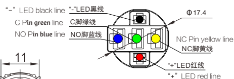
带灯指示 LED
