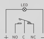
3档原理图 Schematic diagram of 3 gear
