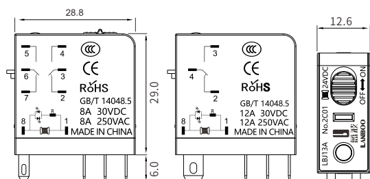
银触点,大电流 Silver contact,High Current
