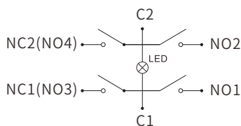
带灯 (3档/6脚) With LED (3rd gear/6-pin)
