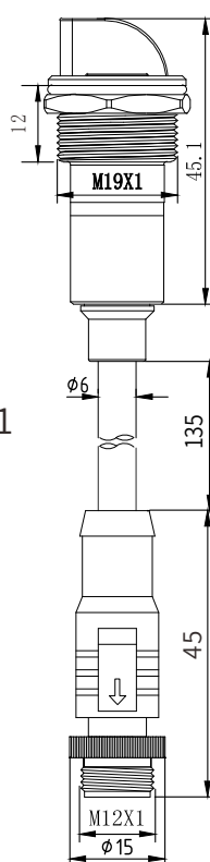
不锈钢外壳, 坚固耐用 stainless steel
