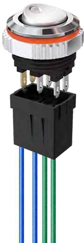
带指示灯 LED
