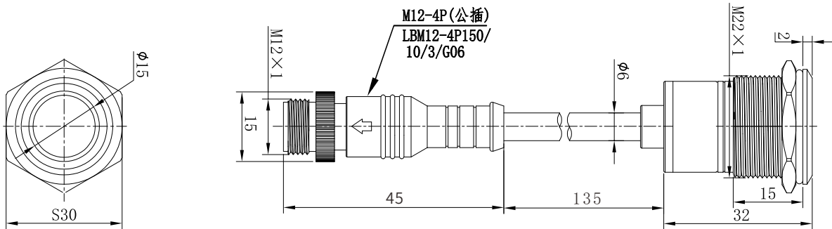
不锈钢外壳, 坚固耐用 stainless steel
