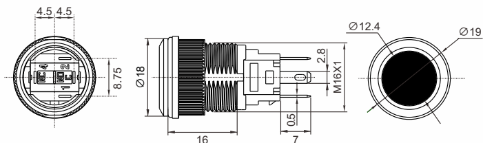
发光面积大,灯光柔和 Whole Face LED
