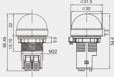
球头指示灯 Ball head indicator light
