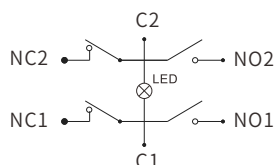
带灯 (2档/6脚) With LED (2 Gears/6 PINS)
