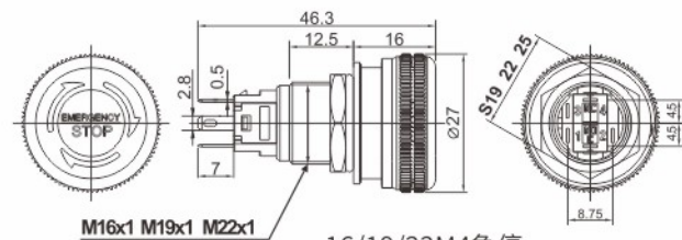
16/19/22M4急停 16/19/22M4 Stop Button
