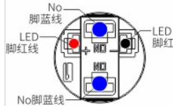
短脚无接插件 Short pin without connector
