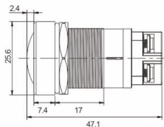
螺丝脚方便接线 Screw Pins
