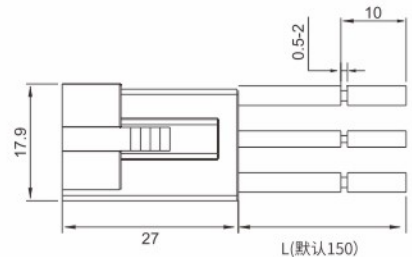
银触点, 加粗银插脚 Big Silver Pins
