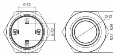
LB19QC LB22QC
