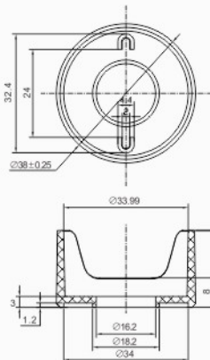
LB16FW-J1-1.1
