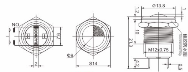
12B外形尺寸 Outline Dimension
