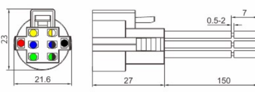
M5.1 M5.2 M5.4专用接插件 Connector
