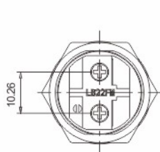
304金属面罩、IP65 304 Stainless Steel, IP65
