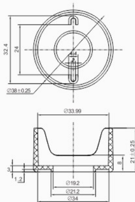
LB19FW-J1-1.1
