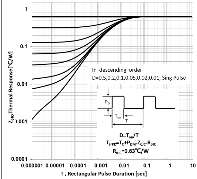
Figure 3a Max Thermal Impedance (TO-220/TO-251/TO-252)
