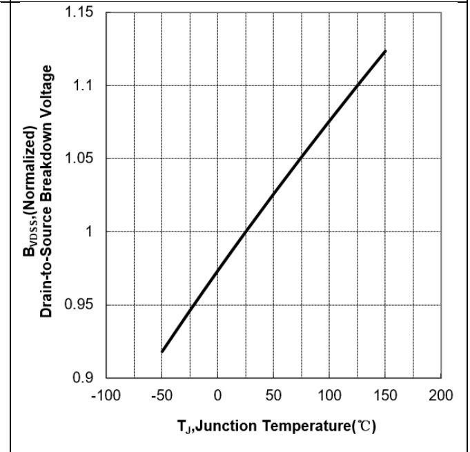
Figure 9 Typical Breakdown Voltage vs Junction Temperature
