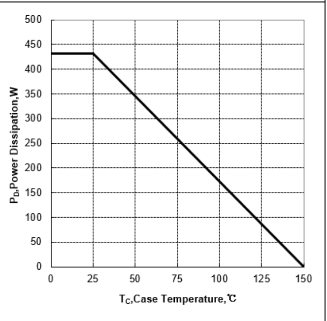
Figure 2 Power Dissipation
