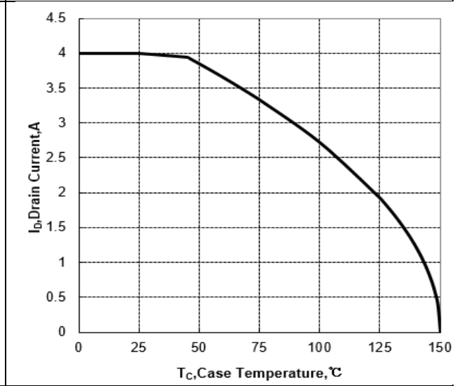
Figure 4 Maximum Continuous Drain Current
