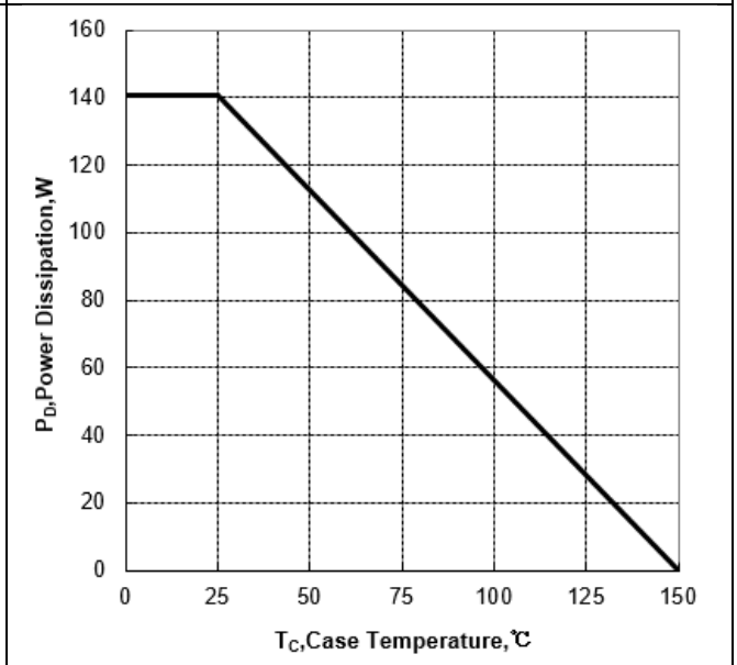
Figure 2a Power Dissipation (TO-220)
