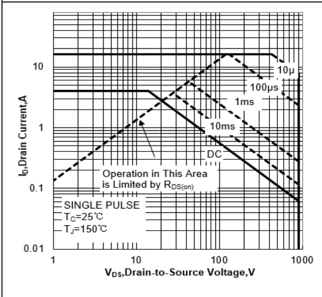
Figure 1c Safe Operating Area (TO-251\TO-252)
