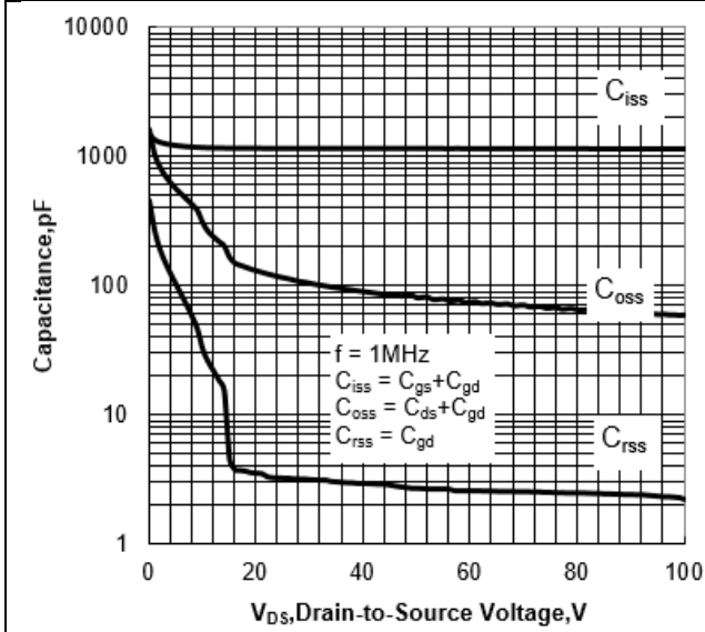
Figure 10 Capacitance Characteristics
