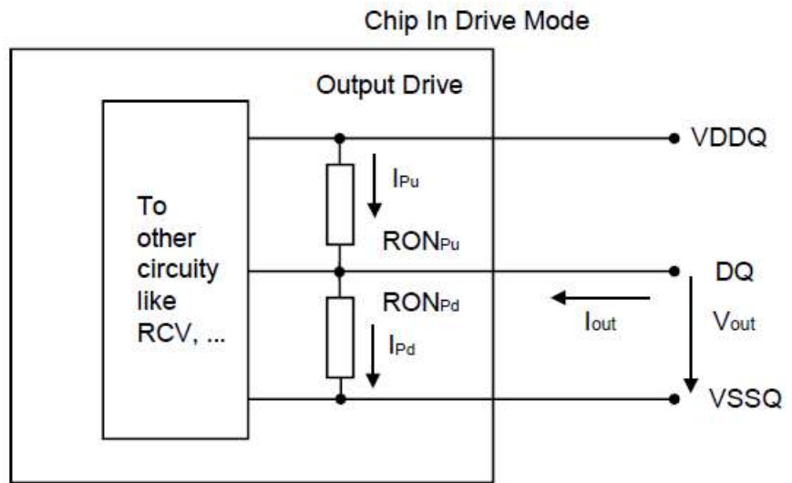
Figure 5-1. Output Driver
