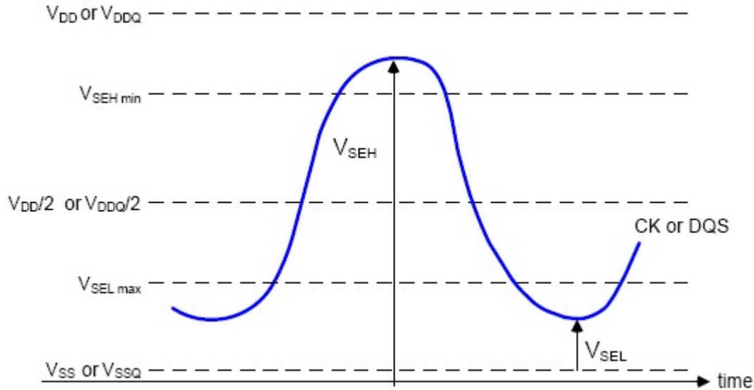
Figure 4-31 Single-ended requirement for differential signals
