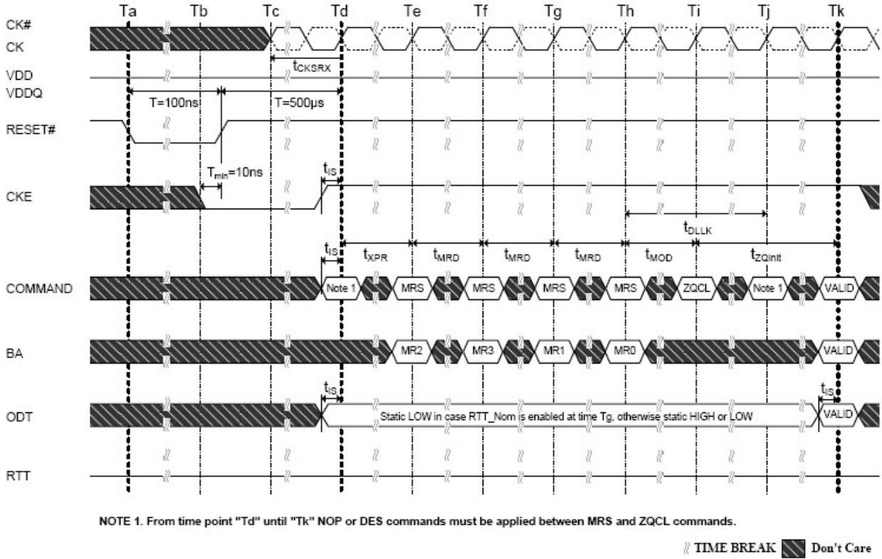
Figure 4-2 Reset Procedure at Power Stable Condition
