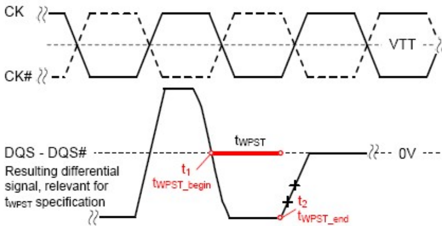
Figure 4-24 Method for calculating t WPST transitions and endpoints
