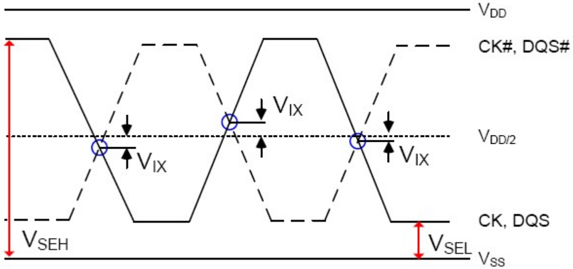
Figure 4-32 Vix Definition
