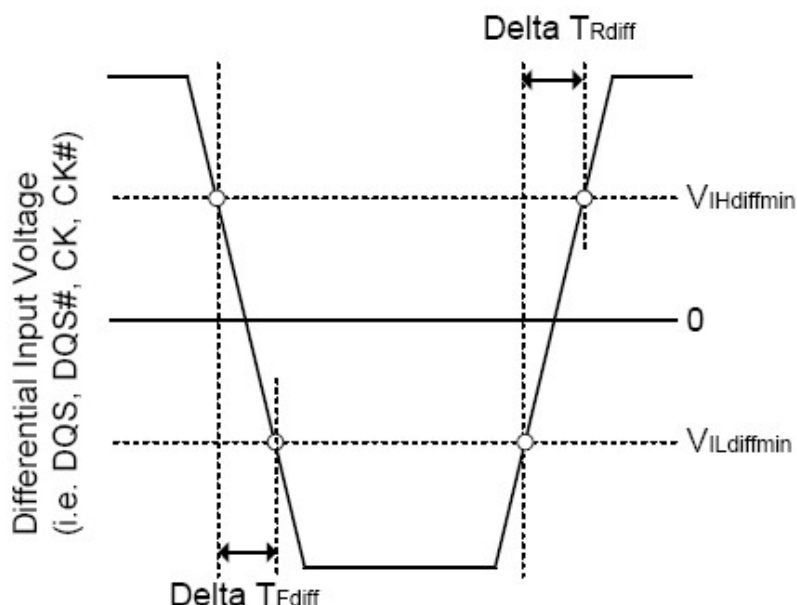
Figure 4-34. Differential Input Slew Rate Definition for DQS, DQS# and CK, CK#
