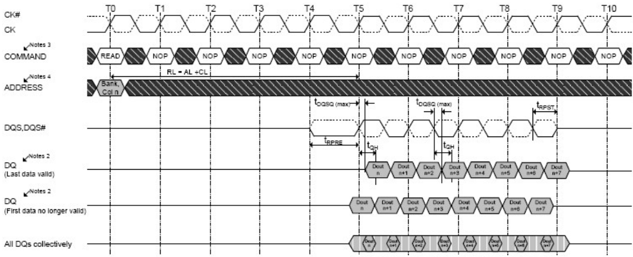
Figure 4-19 Data Strobe to Data Relationship
