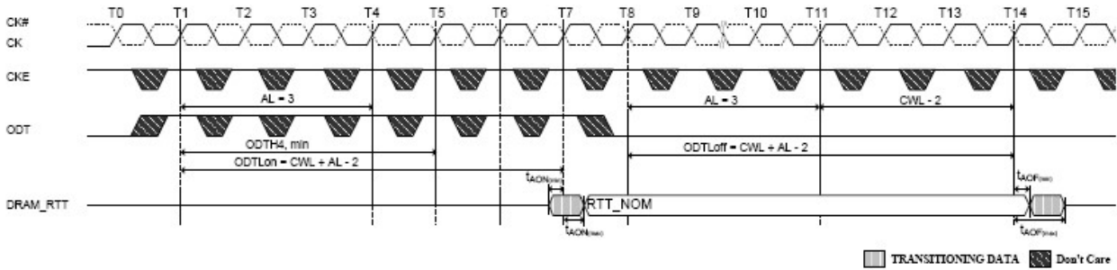
Figure 4-88 Synchronous ODT Timing Example
