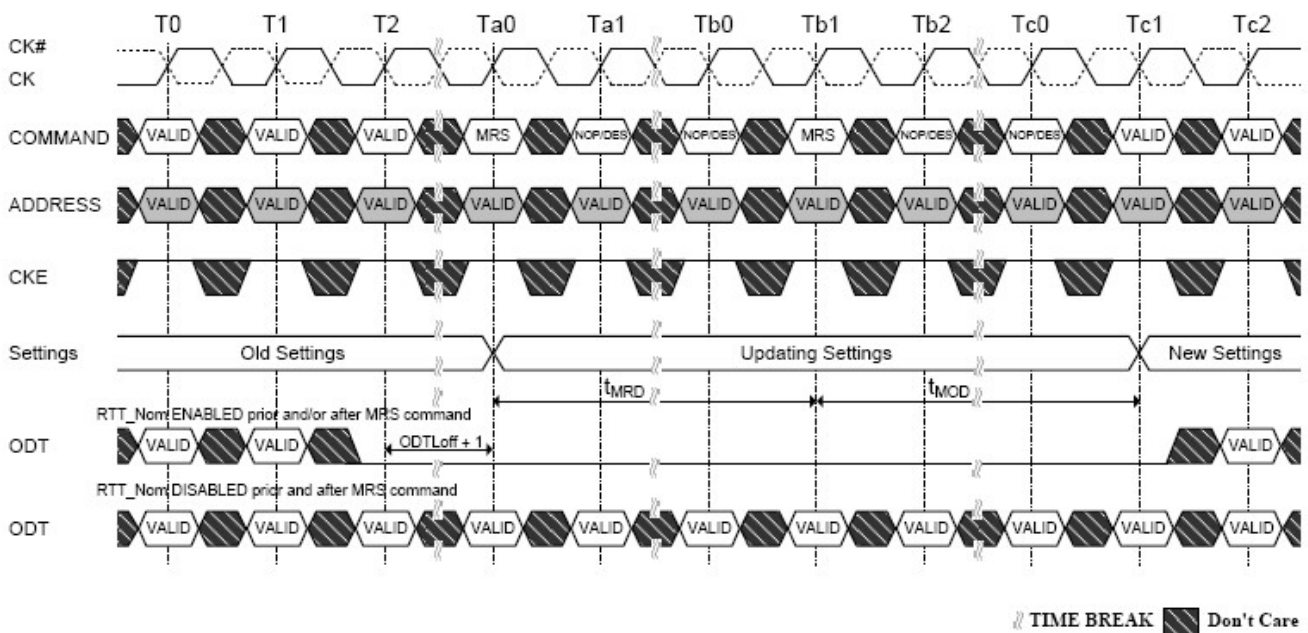
Figure 4-3 tMRD timing
