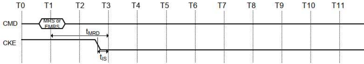
Figure 4-55 MRS/EMRS command to power-down entry
