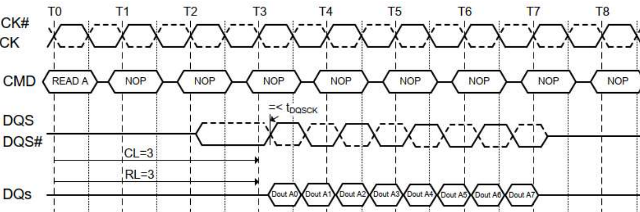
Figure 4-19 Burst read operation: RL=3 (AL=0, CL=3, BL=8)
