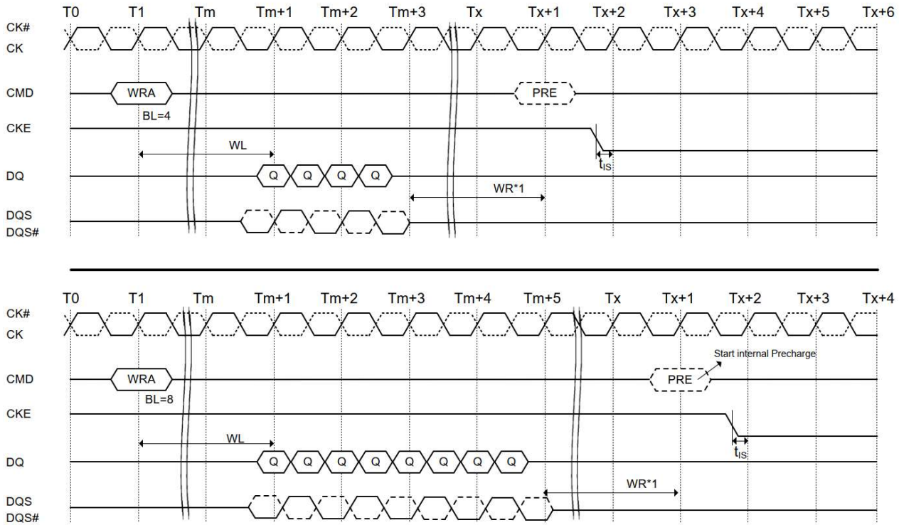
Figure 4-51 Write with autoprecharge to power-down entry
