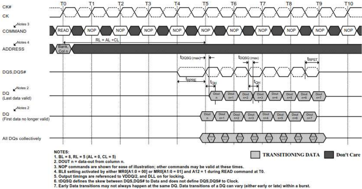
Figure 4-17 Data Strobe to Data Relationship
