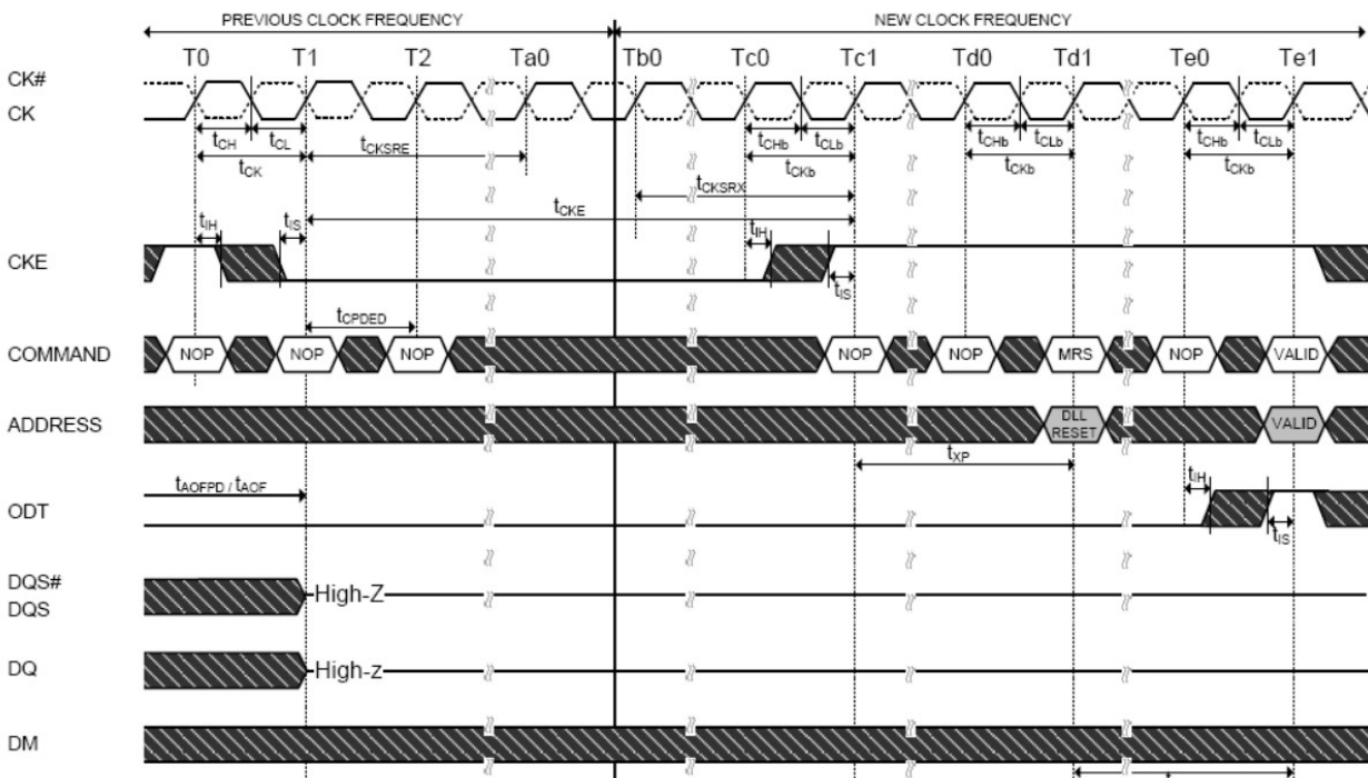
Figure 4-9 Change Frequency during Precharge Power-down
