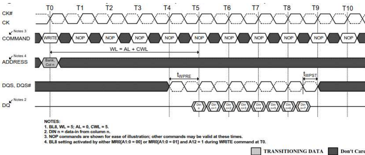
Figure 4-41 WRITE Burst Operation WL = 5 (AL = 0, CWL = 5, BL8)
