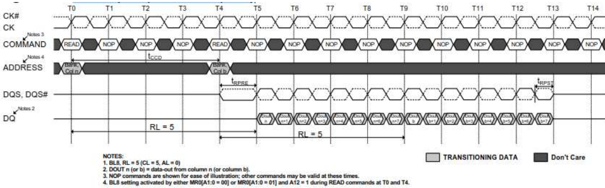
Figure 4-29 READ (BL8) to READ (BL8)
