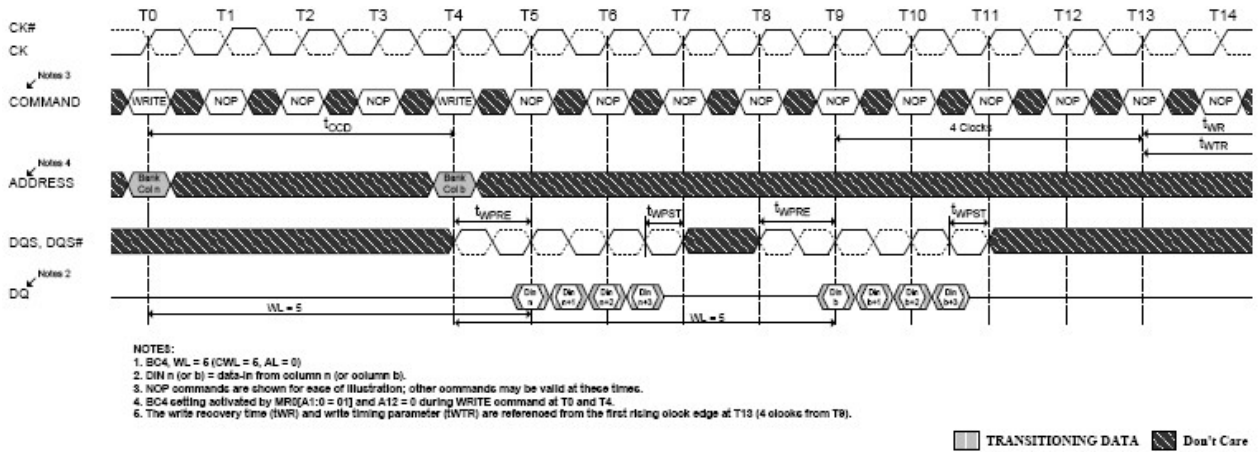
Figure 4-71 WRITE (BC4) to WRITE (BC4) OTF
