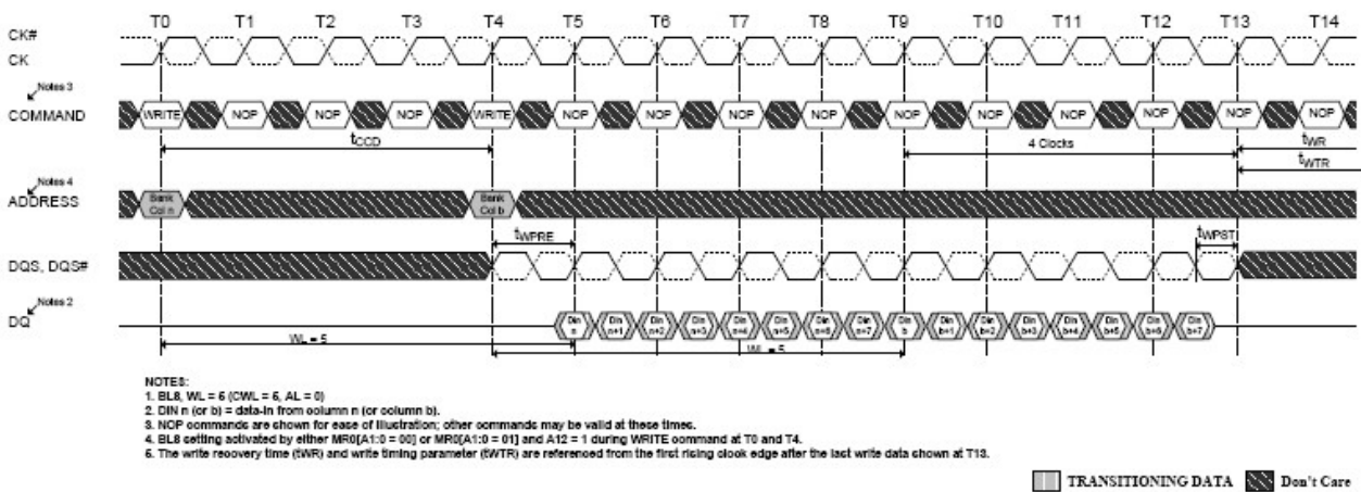
Figure 4-70 WRITE (BC8) to WRITE (BC8)
