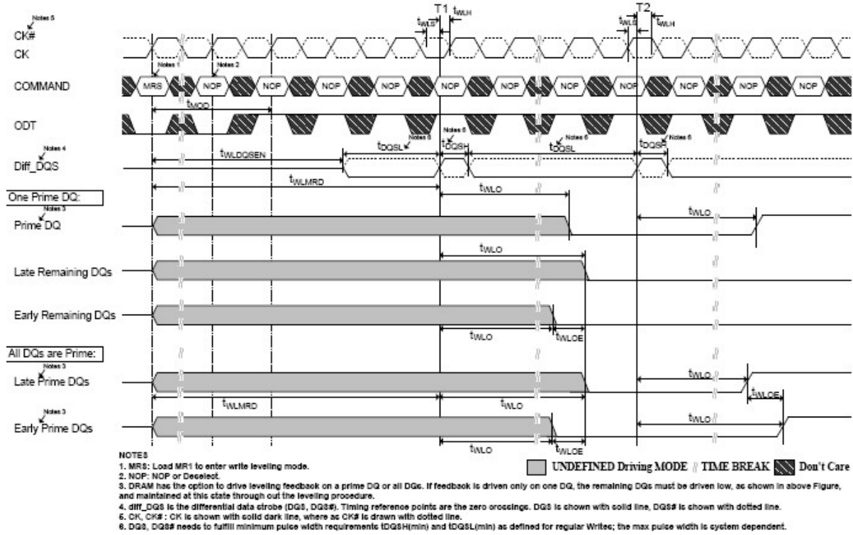
Figure 4-13 Timing details of Write Leveling sequence (DQS – DQS# is capturing CK – CK# low at T1 and CK – CK# high at T2)
