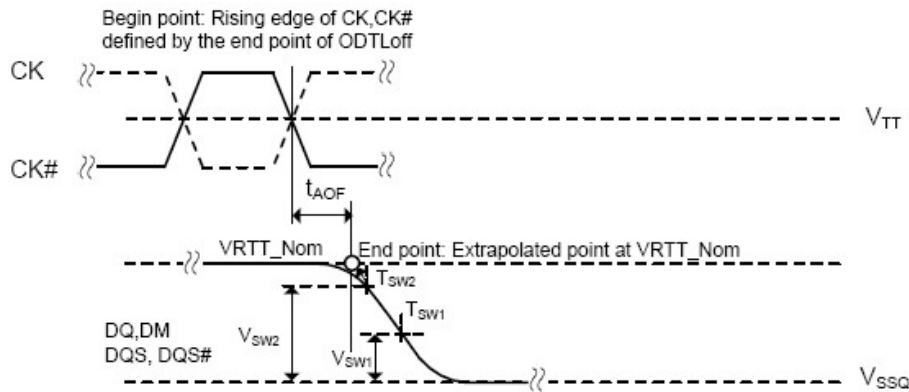
Figure 4-45 Definition of t AOFF
