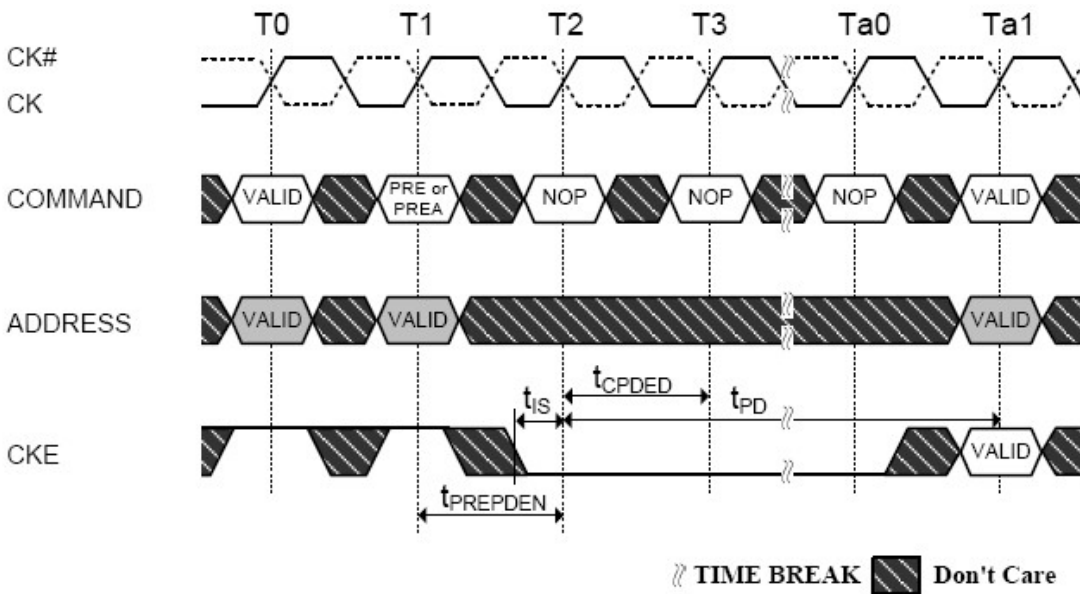
Figure 4-86 Precharge, Precharge all command to Power-Down Entry
