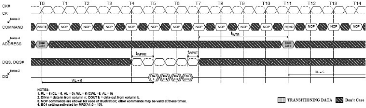
Figure 4-74 WRITE (BC4) to READ (BC4)
