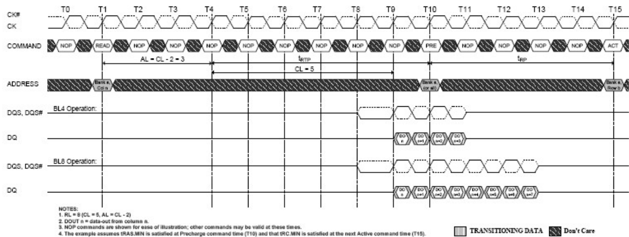
Figure 4-63 READ to PRECHARGE, RL = 8, AL = CL-2, CL = 5, tRTP = 6, tRP = 5
