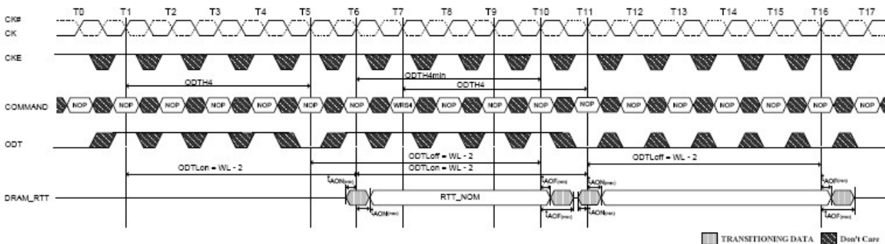
Figure 4-89 Synchronous ODT example with BL = 4, WL = 7
