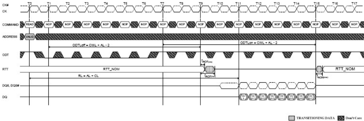
Figure 4-29 ODT must be disabled externally during Reads by driving ODT low (CL=6; AL=CL-1=5; RL=AL+CL=11; CWL=5; ODTLon=CWL+AL-2=8; ODTLoff=CWL+AL-2=8)
