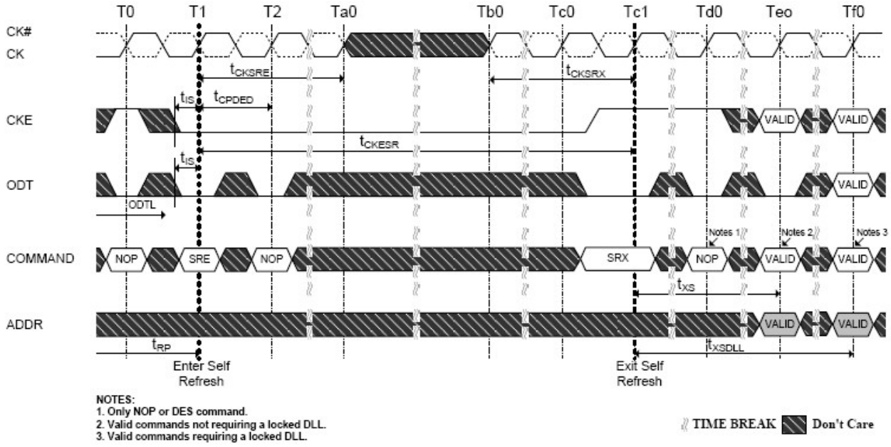
Figure 4-77 Self-Refresh Entry/Exit Timing
