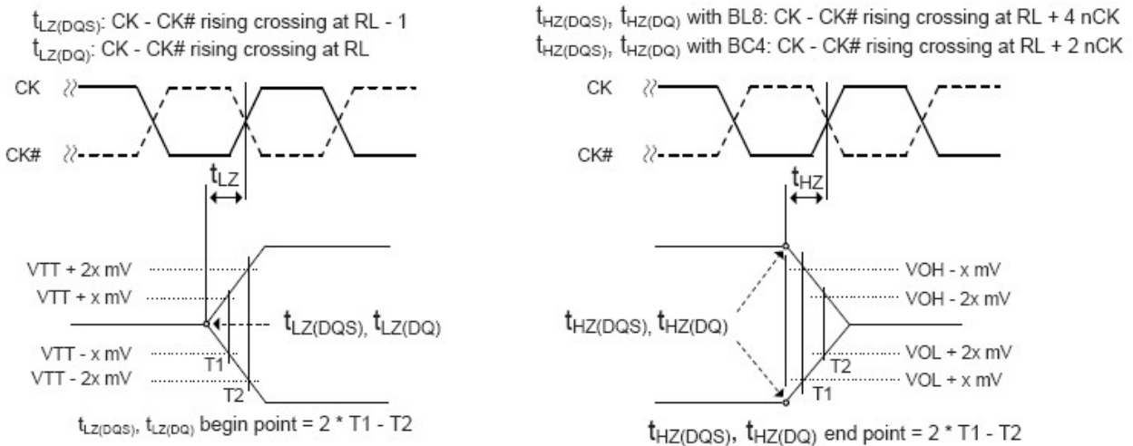
Figure 4-20 tLZ and tHZ method for calculating transitions and endpoints
