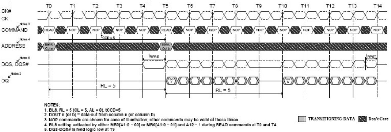
Figure 4-54 Nonconsecutive READ (BL8) to READ (BL8)
