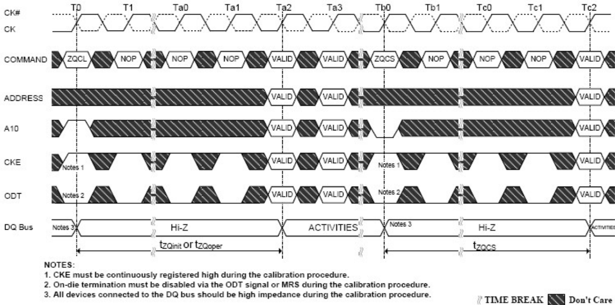
Figure 4-30 ZQ Calibration Timing
