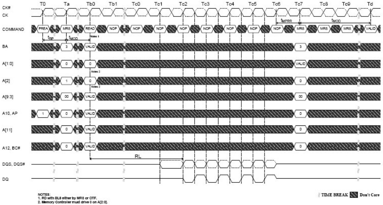
Figure 4-49 MPR Readout of predefined pattern, BL8 fixed burst order, single readout
