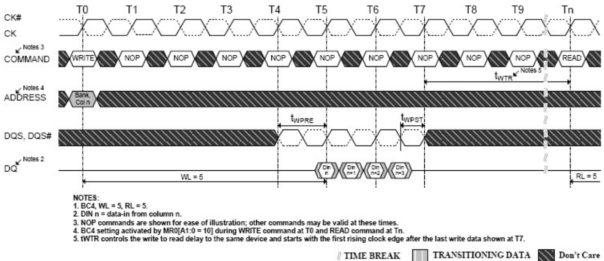
Figure 4-67 WRITE (BC4) to READ (BC4) operation
