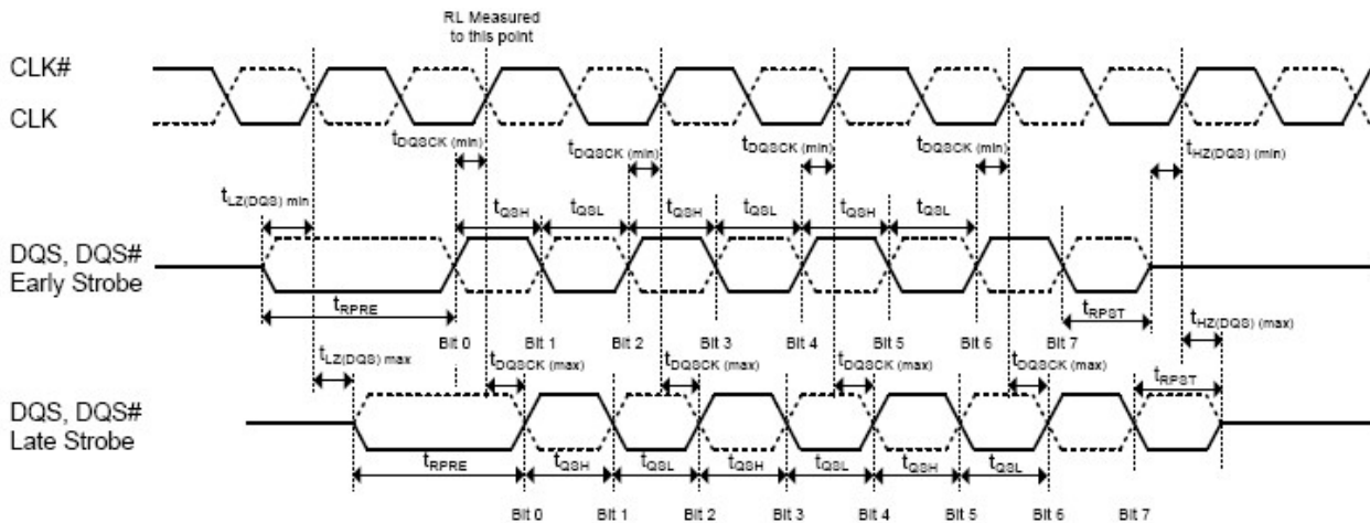
Figure 4-18 Clock to Data Strobe relationship
