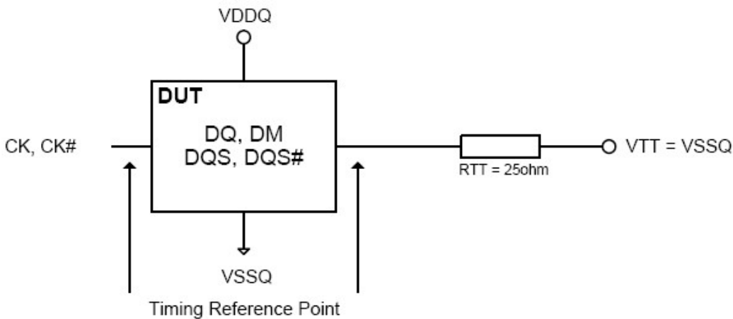
Figure 4-42 ODT Timing Reference Load
