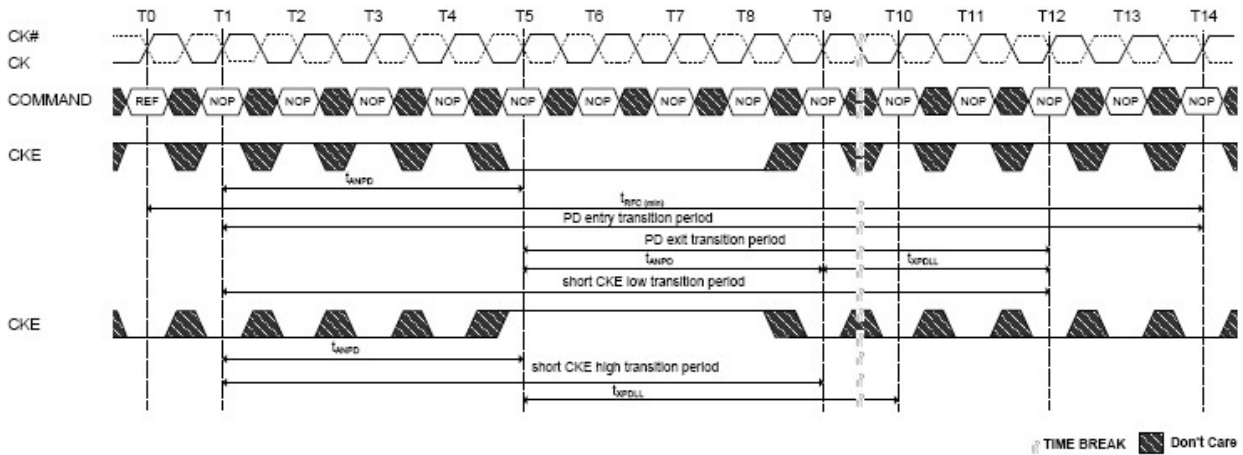
Figure 4-99 Transition period for short CKE cycles, entry and exit period overlapping (AL = 0, WL = 5, tANPD = WL - 1 = 4)
