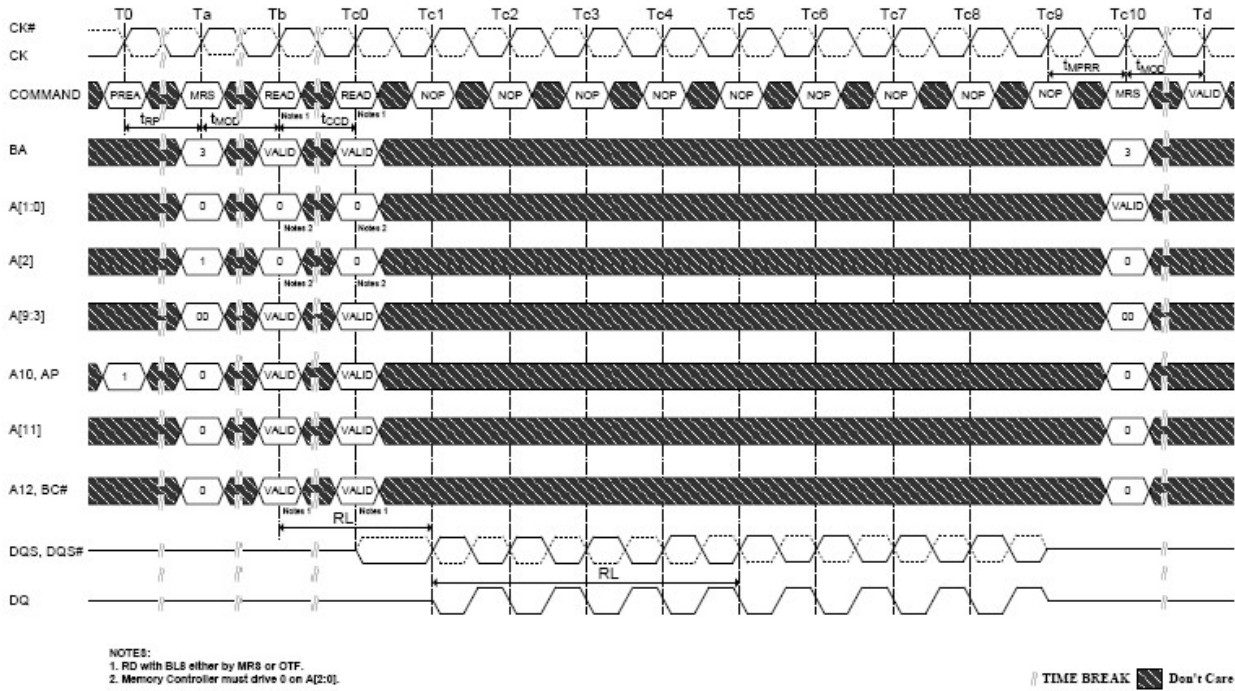
Figure 4-50 MPR Readout of predefined pattern, BL8 fixed burst order, back to back radout
