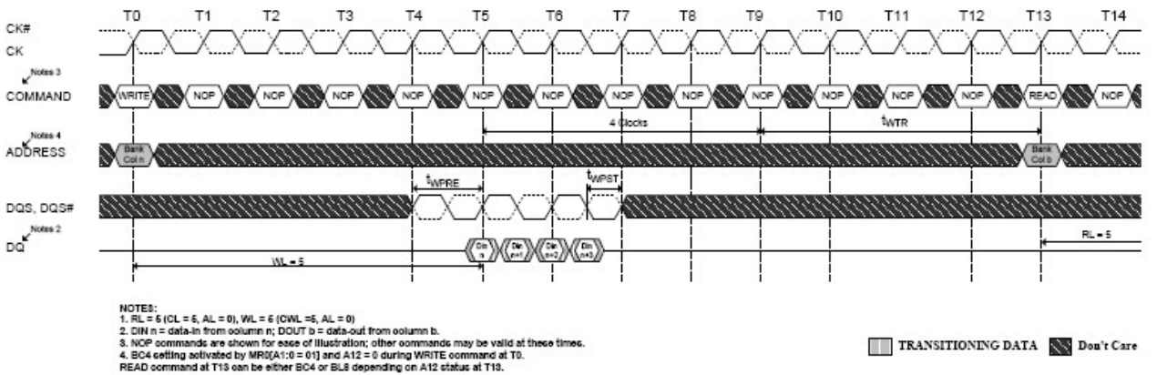
Figure 4-73 WRITE (BC4) to READ (BC4, BC8) OTF
