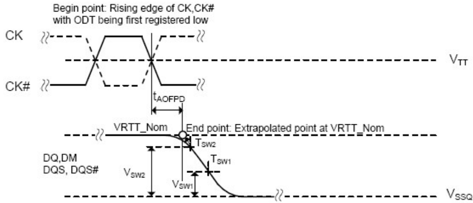
Figure 4-46 Definition of tAOFFPD
