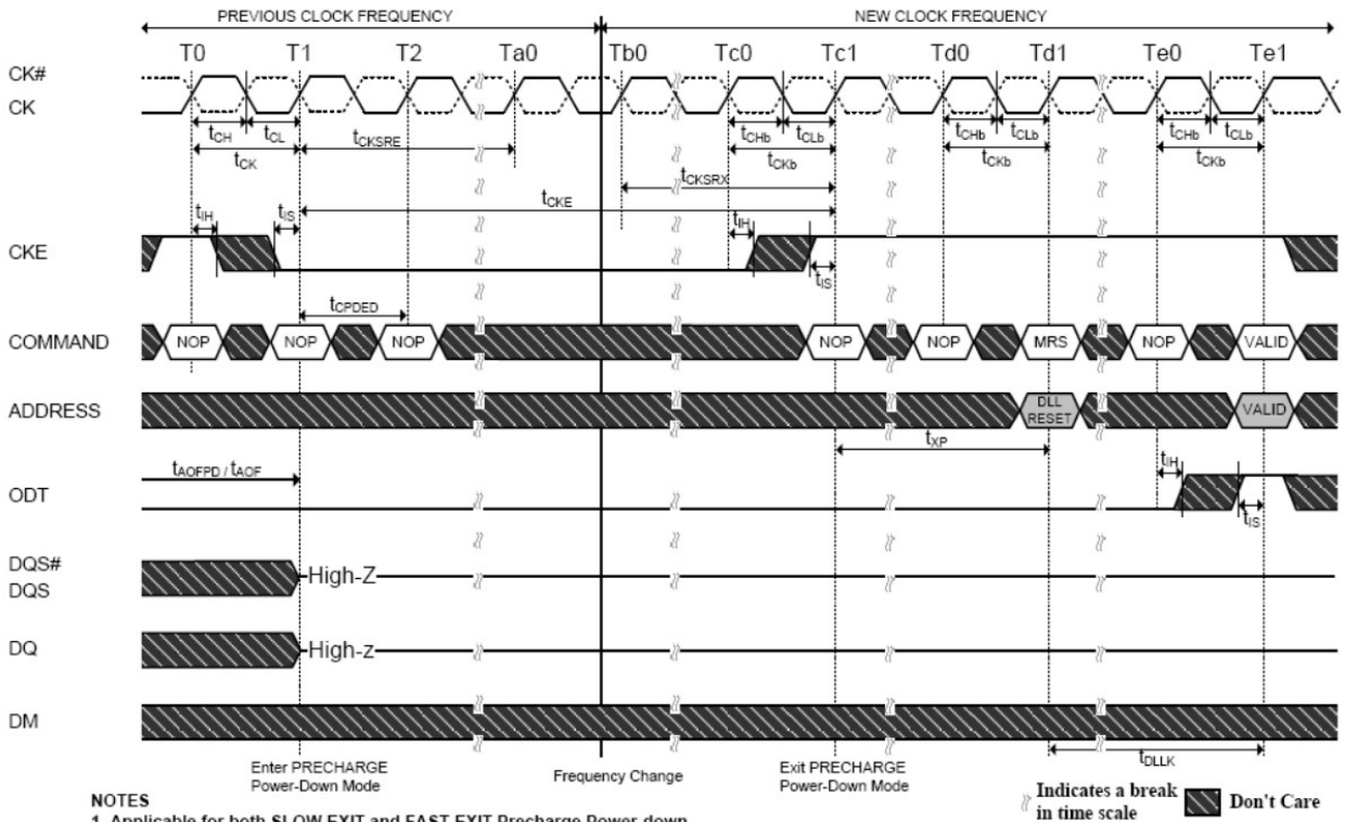
Figure 4-11 Change Frequency during Precharge Power-down
