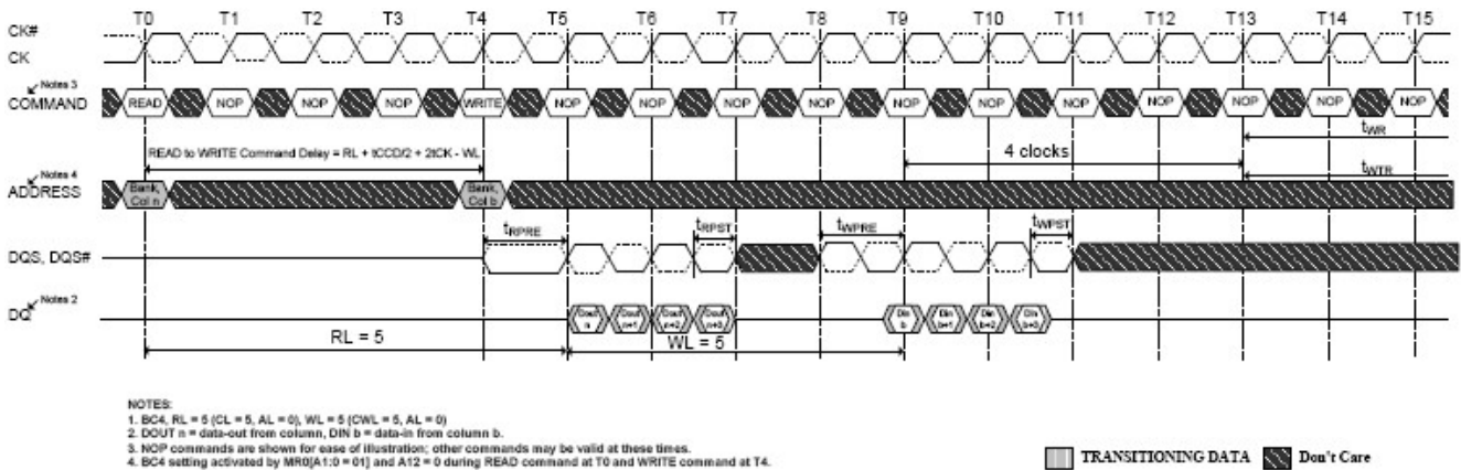
Figure 4-57 READ (BL4) to WRITE (BL4) OTF
