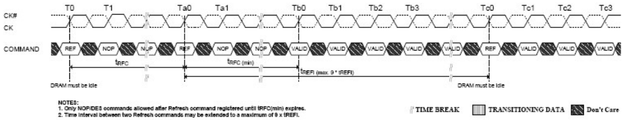
Figure 4-25 Refresh Command Timing
