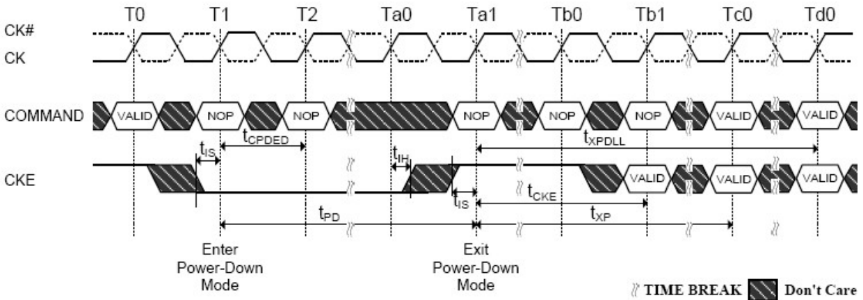
Figure 4-83 Precharge Power-Down (Slow Exit Mode) Entry and Exit
