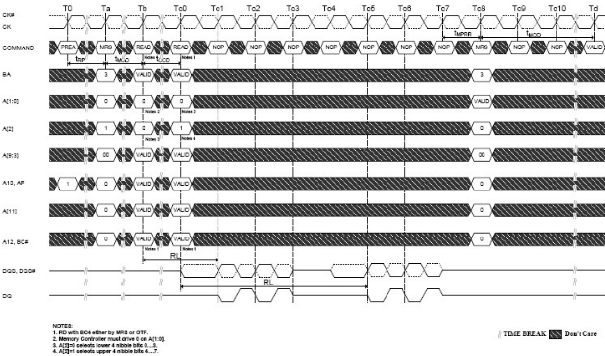
Figure 4-51 MPR Readout of predefined pattern, BC4 lower nibble then upper nibble
