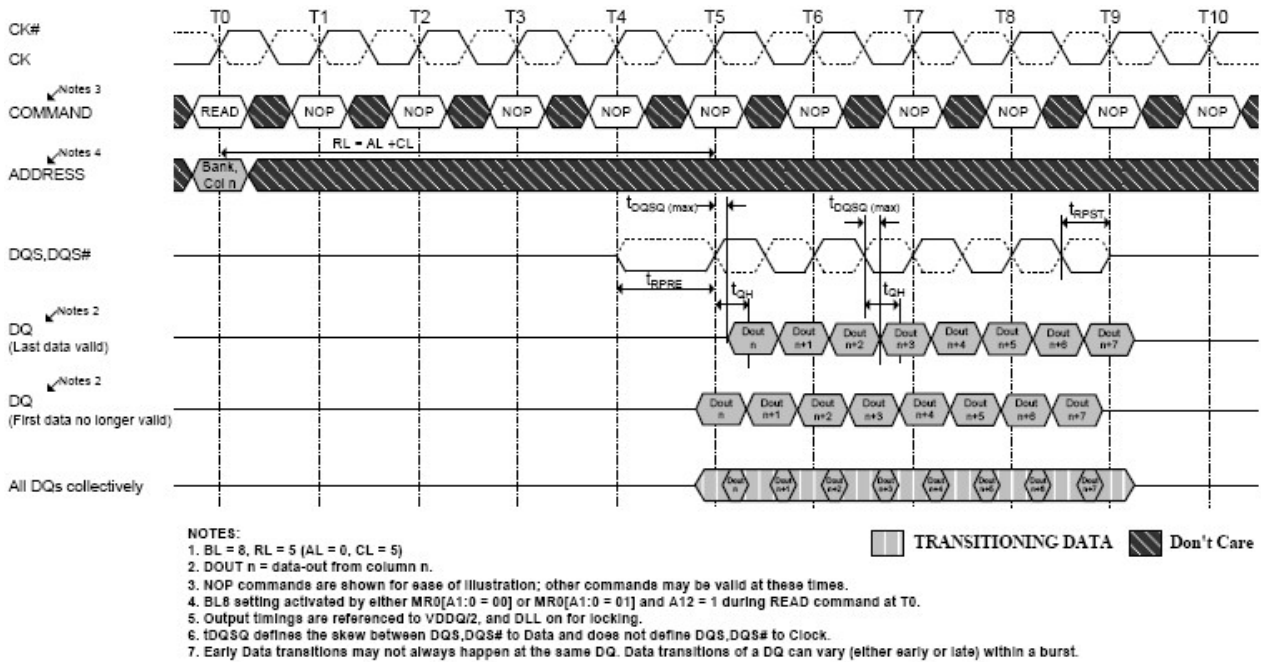
Figure 4-19 Data Strobe to Data Relationship
