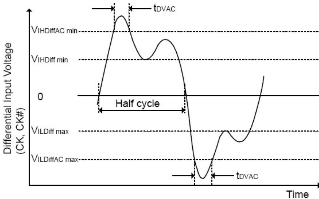
Figure 4-6 Definition of differential ac-swing and “time above ac-level” tDVAC
