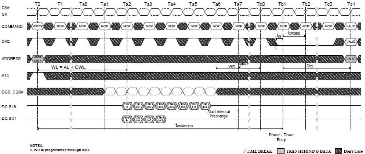
Figure 4-80 Power-Down Entry after Write with Auto Precharge
