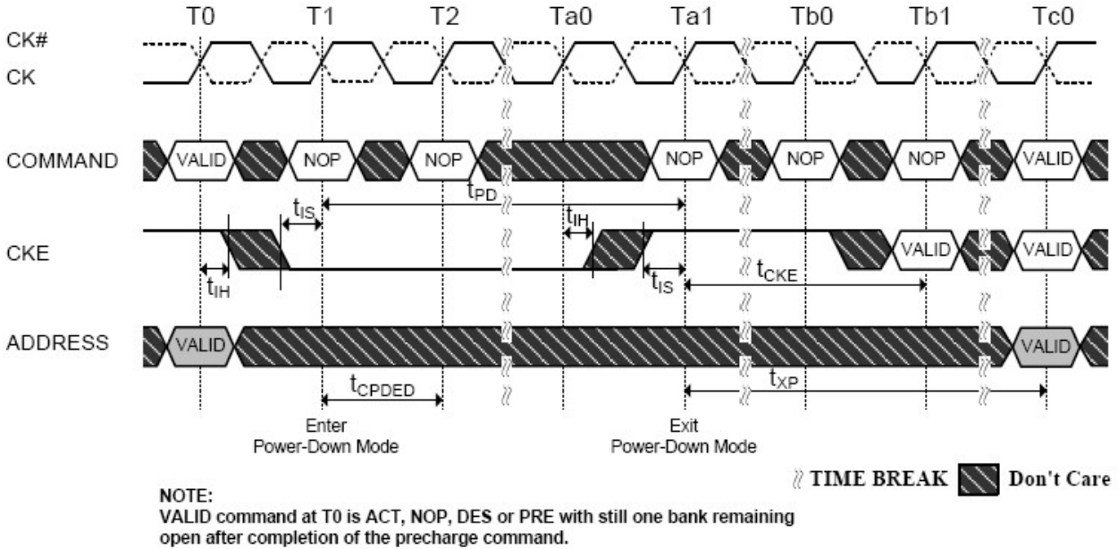
Figure 4-78 Active Power-Down Entry and Exit Timing Diagram
