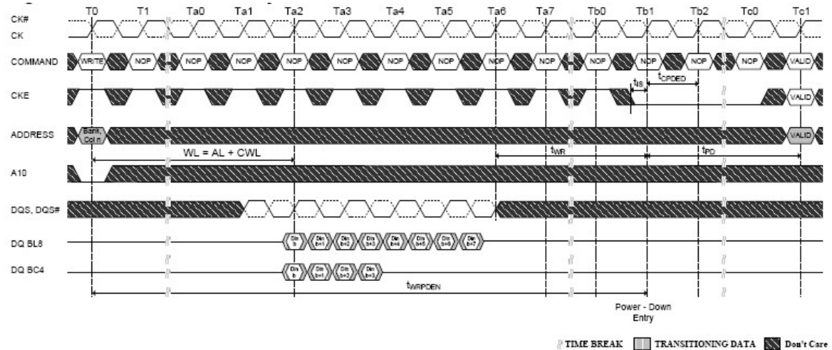
Figure 4-81 Power-Down Entry after Write
