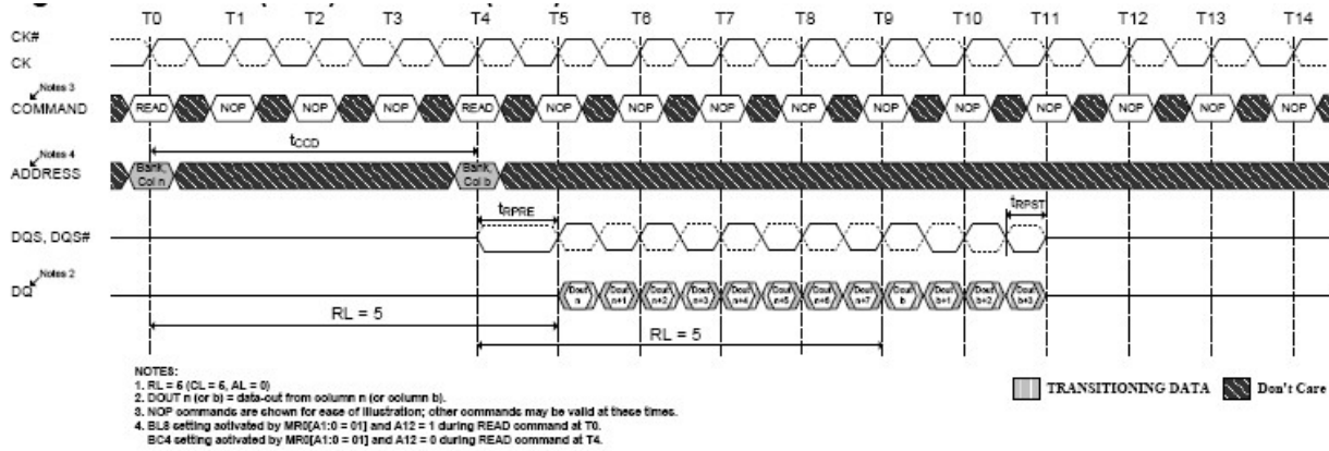
Figure 4-58 READ (BL8) to READ (BL4) OTF
