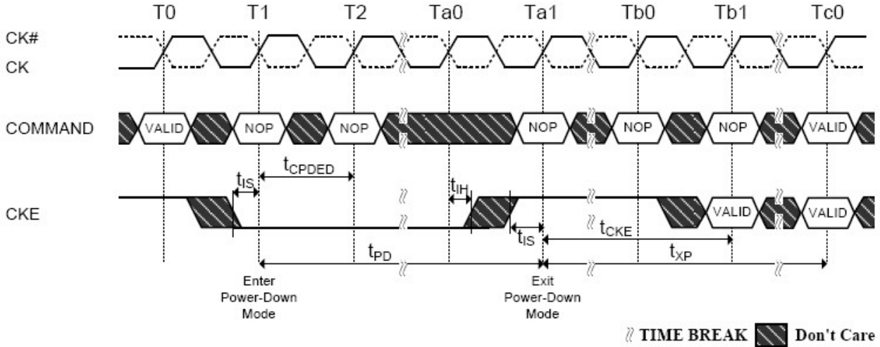
Figure 4-82 Precharge Power-Down (Fast Exit Mode) Entry and Exit
