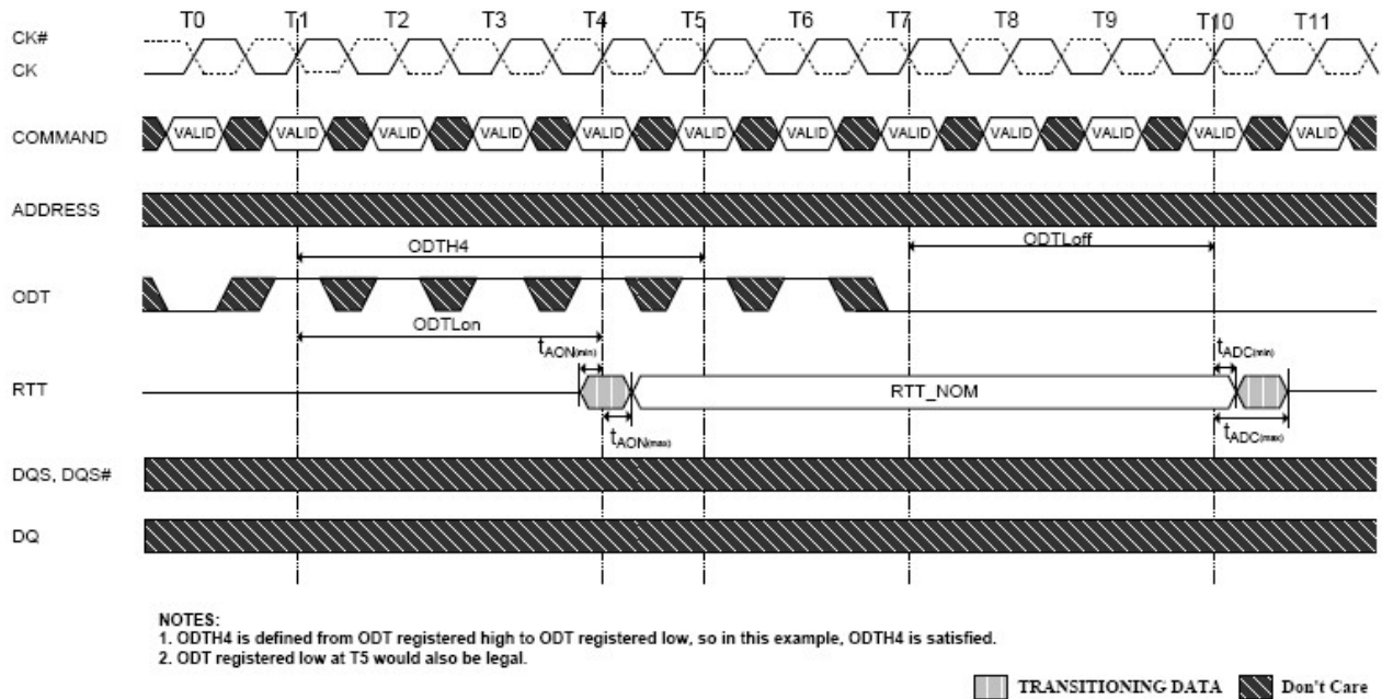
Figure 4-91 Dynamic ODT: Behavior without write command, AL = 0, CWL = 5
