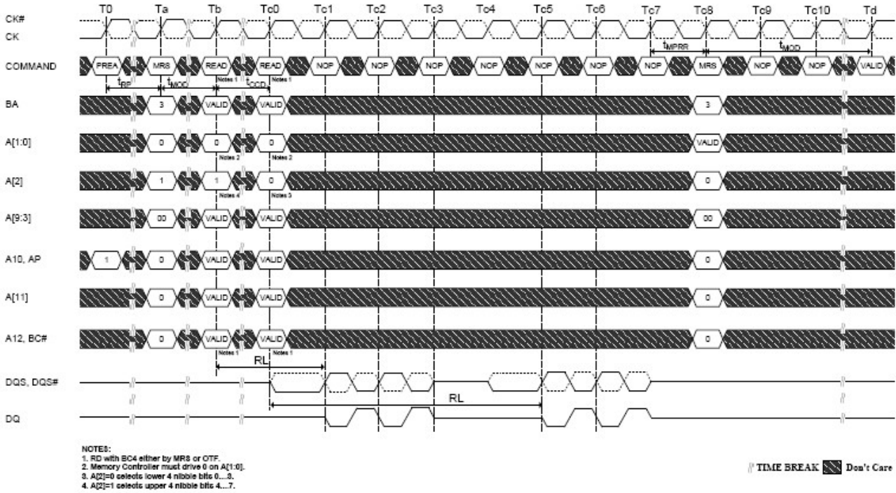
Figure 4-52 MPR Readout of predefined pattern, BC4 upper nibble then lower nibble
