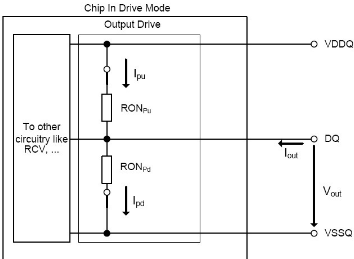
Figure 4-40 Output Driver: Definition of Voltages and Currents
