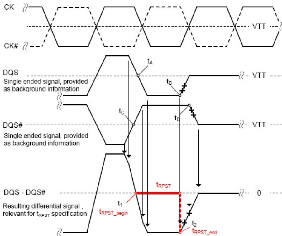
Figure 4-22 Method for calculating t RPST transitions and endpoints
