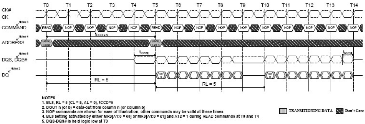
Figure 4-56 READ (BL8) to WRITE (BL8)
