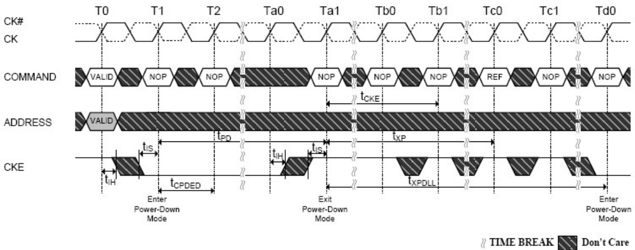
Figure 4-101 Power-Down Entry, Exit Clarifications-Case 2
