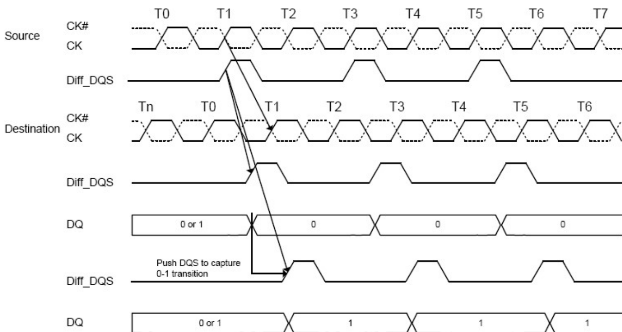
Figure 4-12 Write Leveling Concept
