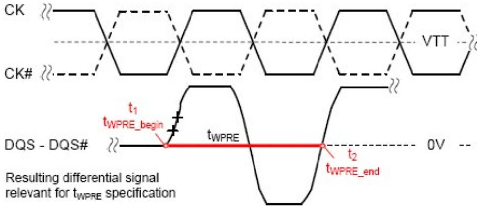
Figure 4-23 Method for calculating t WPRE transitions and endpoints
