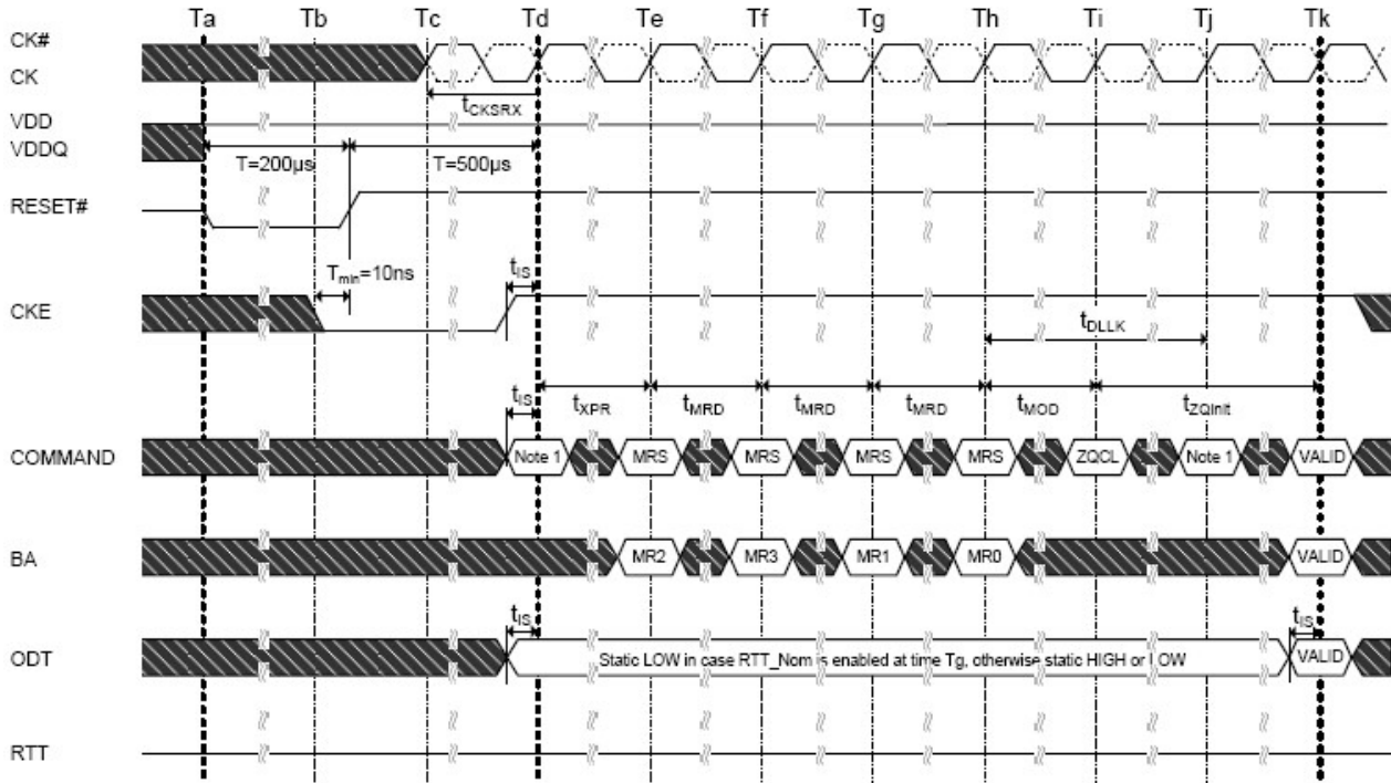
Figure 4-1 Reset and Initialization Sequence at Power-on Ramping
