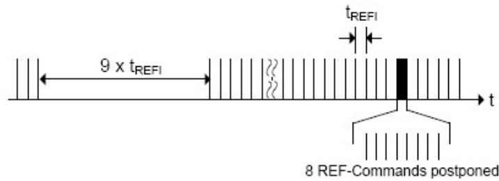
Figure 4-26 Postponing Refresh Commands (Example)
