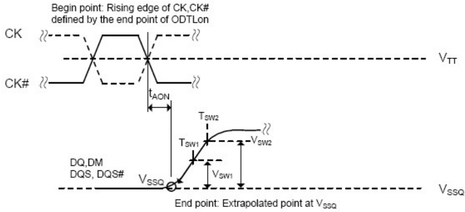
Figure 4-43 Definition of t AON
