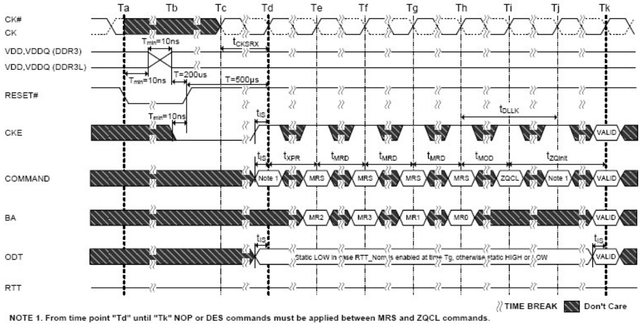
Figure 4-48 MPR Block Diagram VDDQ/VDDQ Voltage Switch Between DDR3L and DDR3
