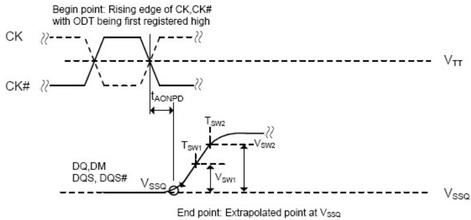
Figure 4-44 Definition of t AONPD
