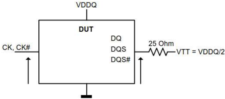
Figure 4-37 Reference Load for AC Timing and Output Slew Rate
