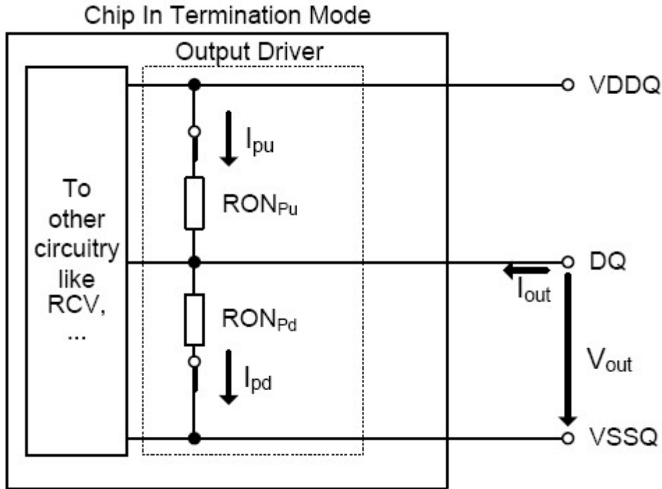
Figure 4-41 On-Die Termination: Definition of Voltages and Currents
