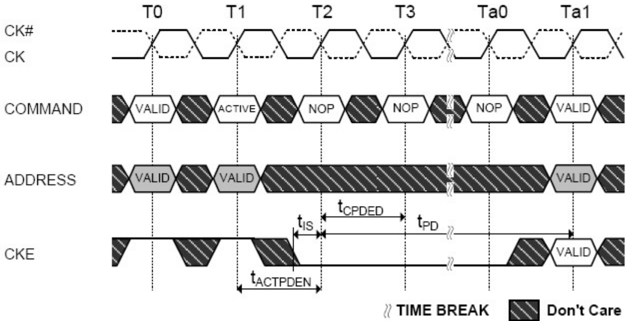
Figure 4-85 Active Command to Power-Down Entry
