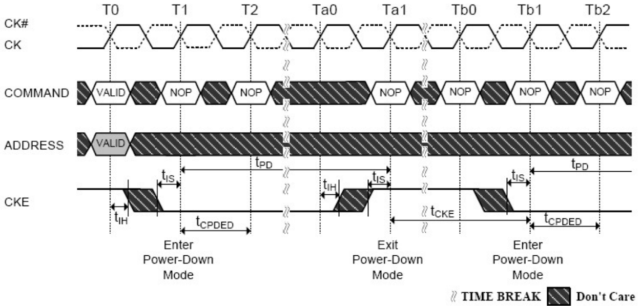
Figure 4-100 Power-Down Entry, Exit Clarifications-Case 1
