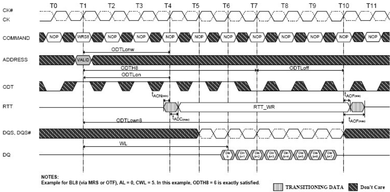
Figure 4-92 Dynamic ODT: Behavior with ODT pin being asserted together with write command for a duration of 6 clock cycles
