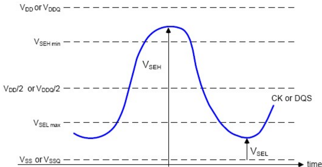
Figure 4-31 Single-ended requirement for differential signals
