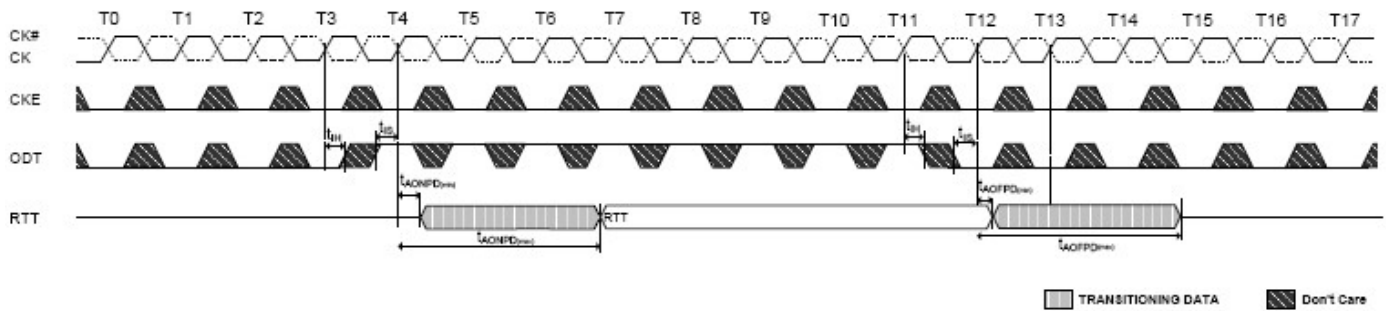
Figure 4-95 Asynchronous ODT Timings on DDR3L SDRAM with fast ODT transition
