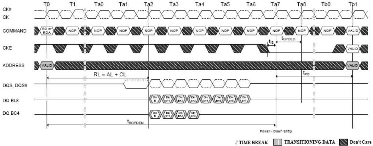
Figure 4-79 Power-Down Entry after Read and Read with Auto Precharge
