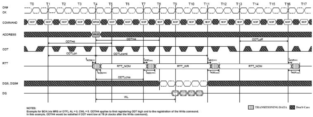
Figure 4-90 Dynamic ODT Behavior with ODT being asserted before and after the write
