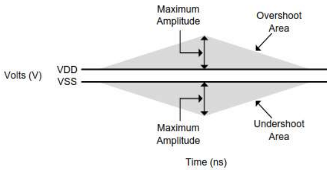
Figure 4-38 AC Overshoot/Undershoot Specification for Address and Control Pins
