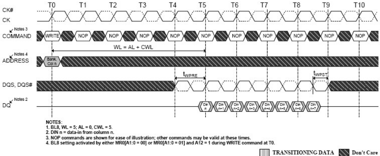
Figure 4-65 WRITE Burst Operation WL = 5 (AL = 0, CWL = 5, BL8)
