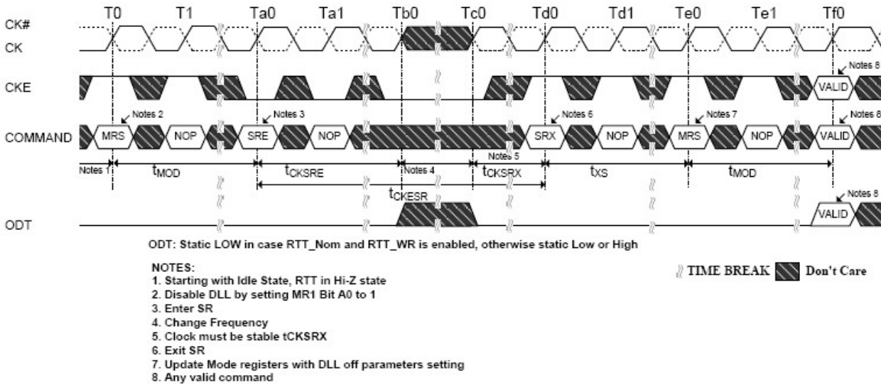
Figure 4-9 DLL Switch Sequence from DLL-on to DLL-off
