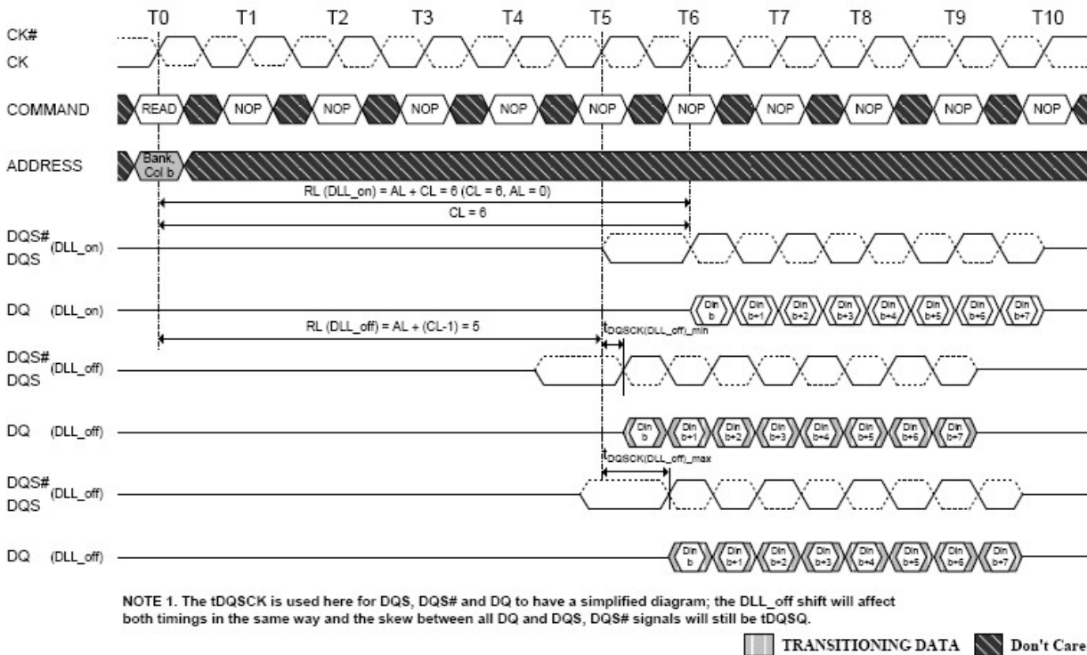
Figure 4-8 DLL-off mode READ Timing Operation
