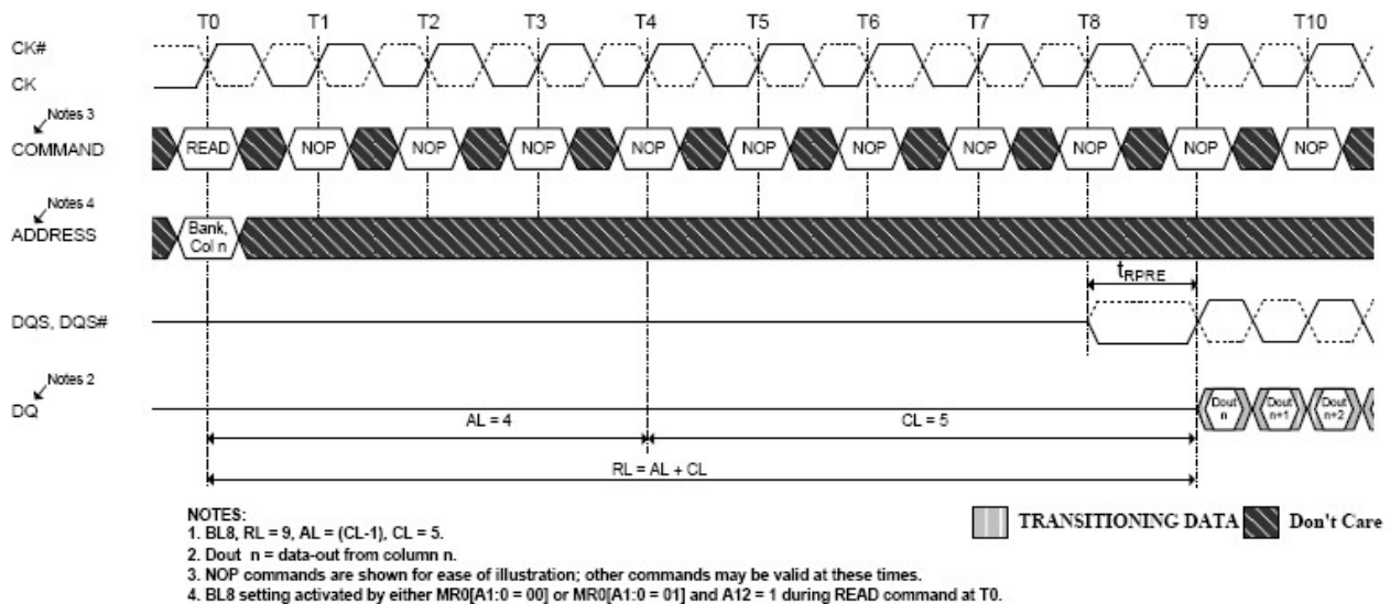
Figure 4-16 READ Burst Operation RL=9 (AL=4, CL=5, BL=8)
