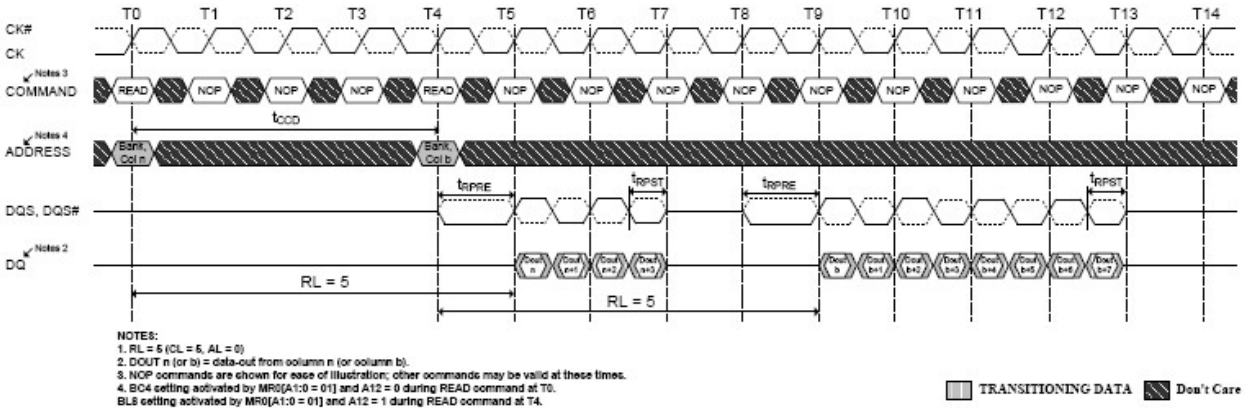
Figure 4-59 READ (BL4) to READ (BL8) OTF
