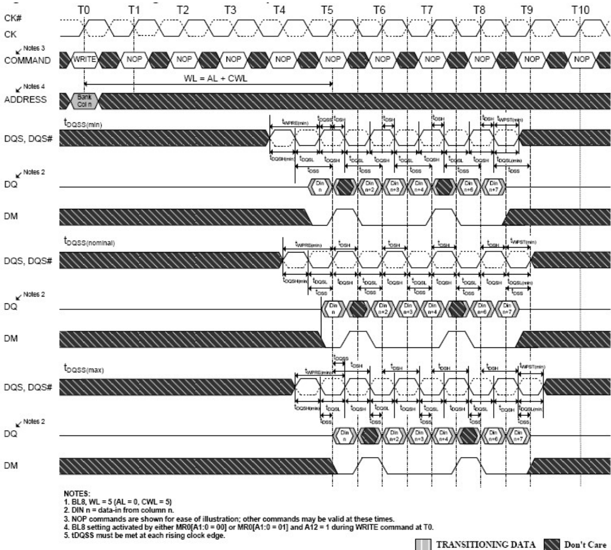
Figure 4-64 Write Timing Definition and parameters
