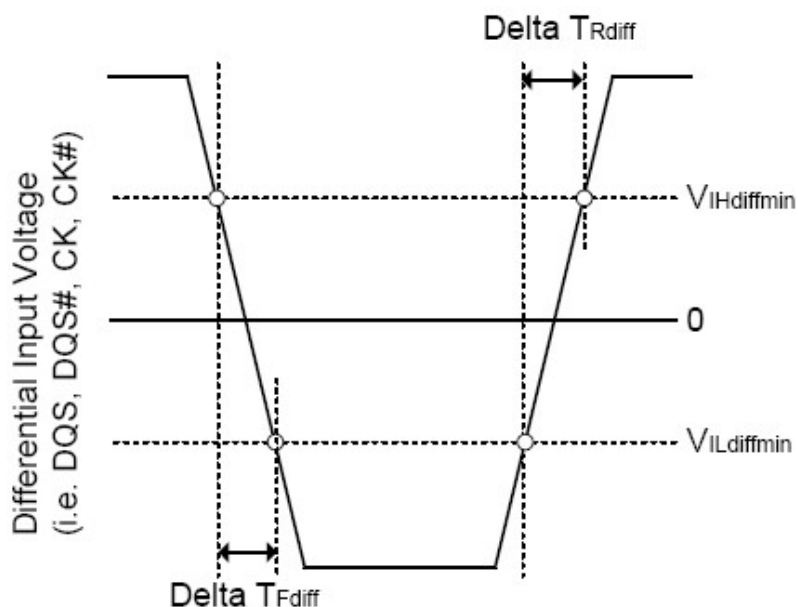
Figure 4-34. Differential Input Slew Rate Definition for DQS, DQS# and CK, CK#
