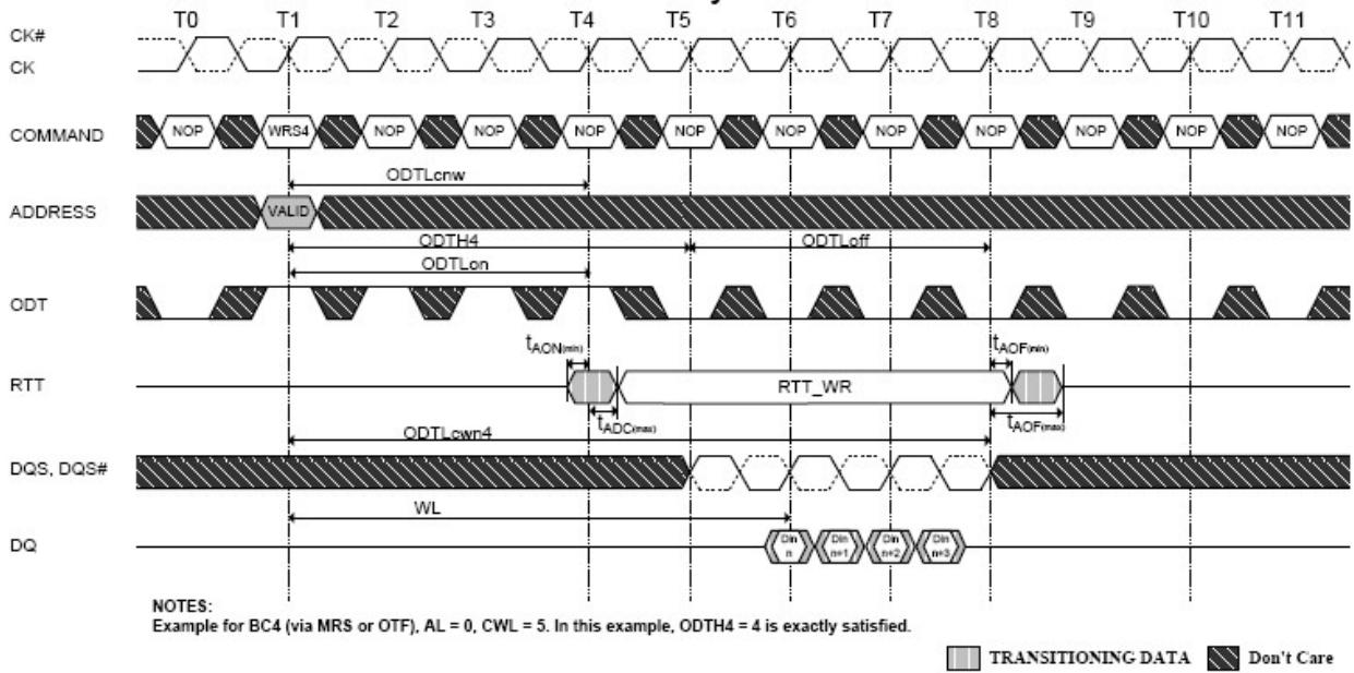
Figure 4-94 Dynamic ODT: Behavior with ODT pin being asserted together with write command for a duration of 4 clock cycles
