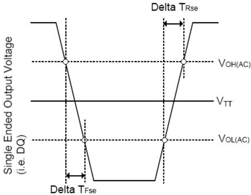
Figure 4-35 Single-ended Output Slew Rate Definition
