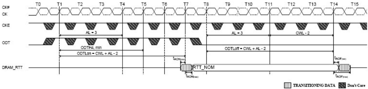
Figure 4-88 Synchronous ODT Timing Example
