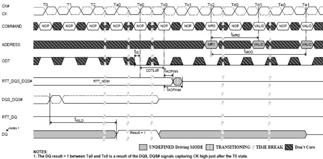
Figure 4-14 Timing details of Write Leveling exit
