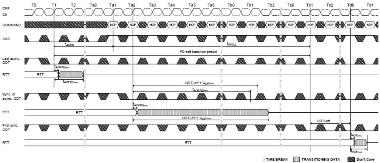
Figure 4-98 Asynchronous to synchronous transition during Precharge Power Down (with DLL frozen) exit (CL = 6; AL = CL - 1; CWL = 5; tANPD = WL - 1 = 9)
