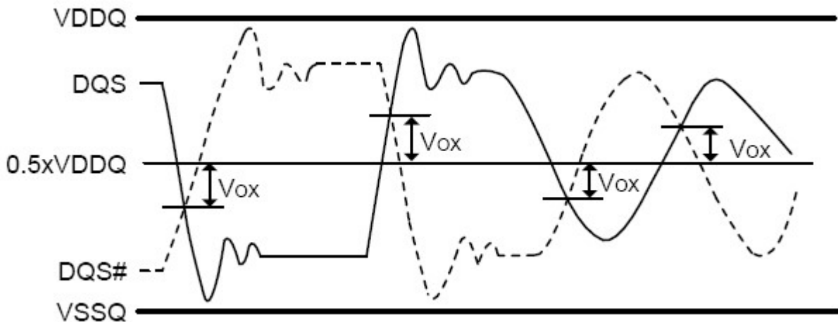
Figure 4-33 Definition of Output cross point voltage for DQS and DQS#
