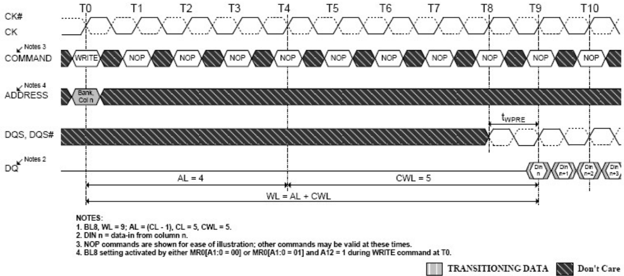
Figure 4-66 WRITE Burst Operation WL = 9 (AL = CL-1, CWL = 5, BL8)
