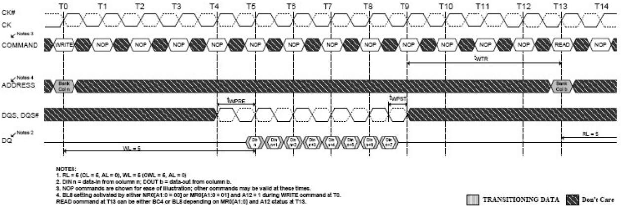
Figure 4-72 WRITE (BC8) to READ (BC4, BC8) OTF
