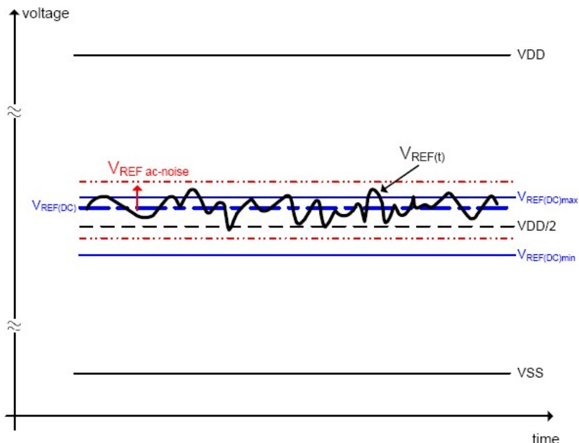
Figure 4-5 Illustration of VREF(DC) tolerance and VREF ac-noise limits
