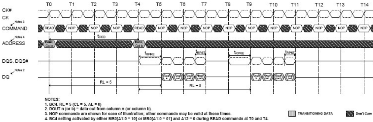
Figure 4-55 READ (BL4) to READ (BL4)
