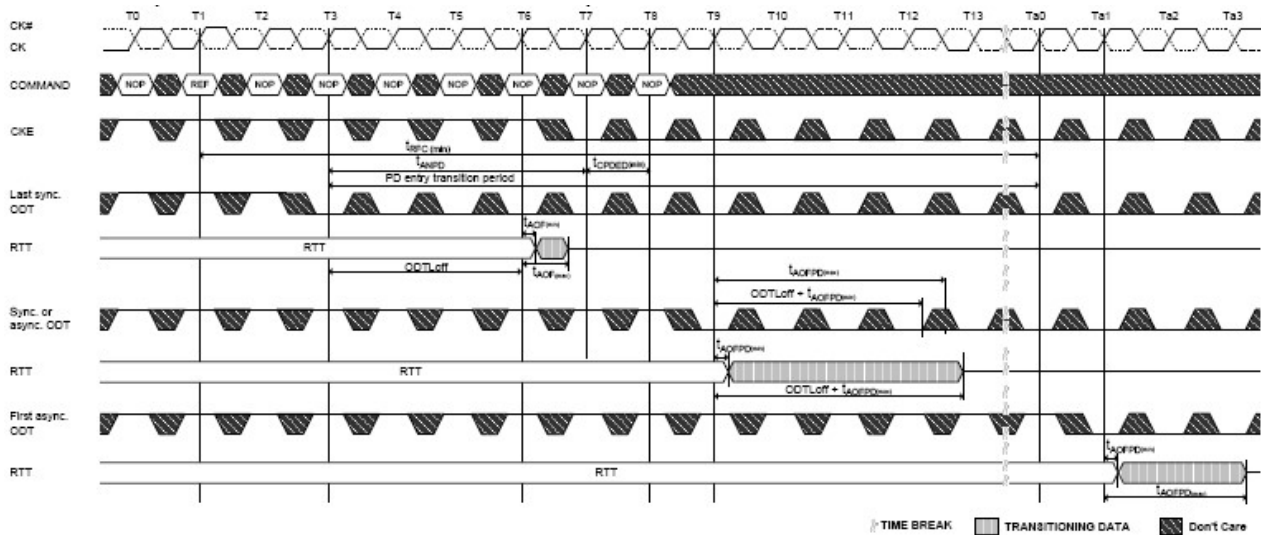
Figure 4-97 Synchronous to asynchronous transition after Refresh command
