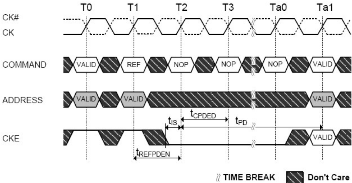
Figure 4-84 Refresh Command to Power-Down Entry
