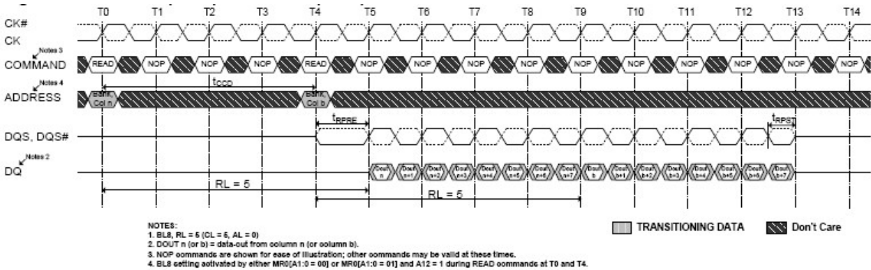
Figure 4-53 READ (BL8) to READ (BL8)
