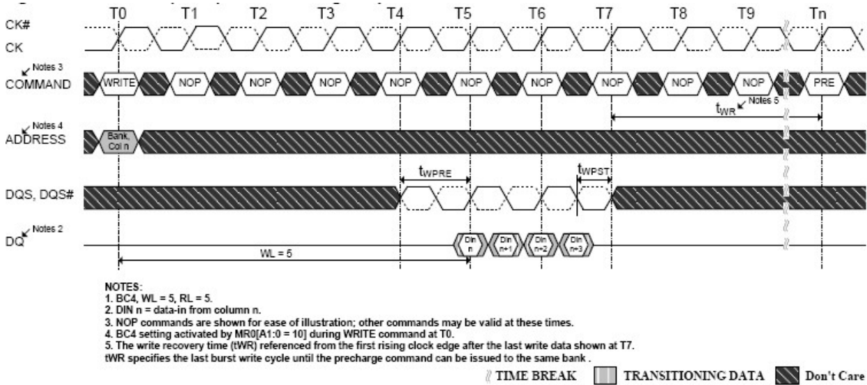
Figure 4-68 WRITE (BC4) to Precharge Operation
