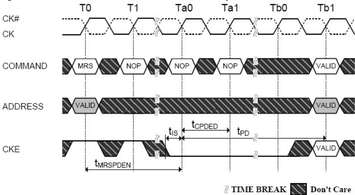
Figure 4-87 MRS Command to Power-Down Entry
