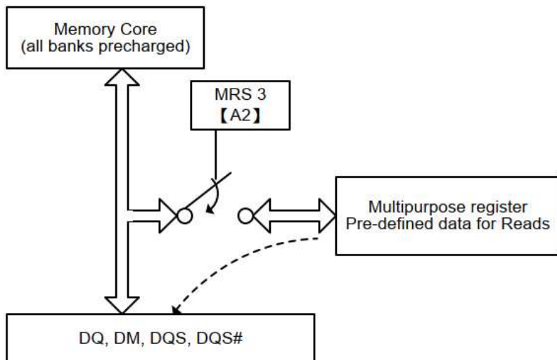
Figure 4-7 MPR Block Diagram
