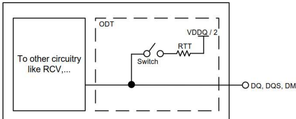
Figure 4-28 Functional representation of ODT
