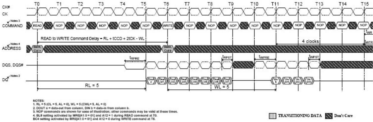
Figure 4-61 READ (BL8) to WRITE (BL4) OTF
