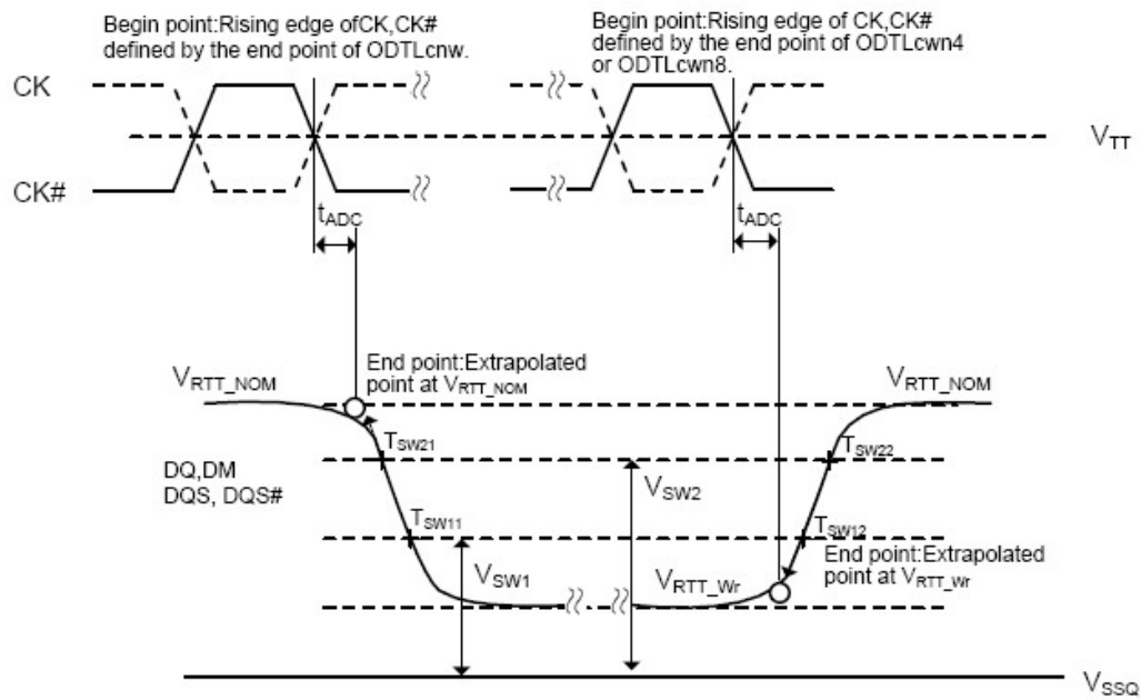
Figure 4-47 Definition of tADC
