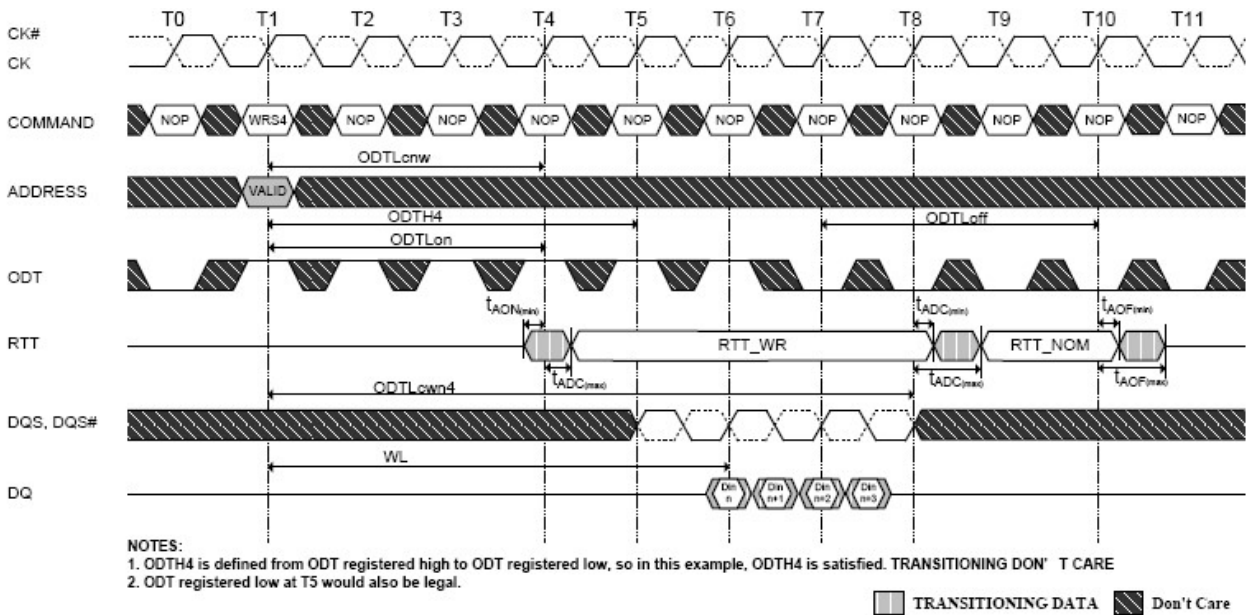
Figure 4-93 Dynamic ODT: Behavior with ODT pin being asserted together with write command for a duration of 6 clock cycles, example for BC4 (via MRS or OTF), AL = 0, CWL = 5
