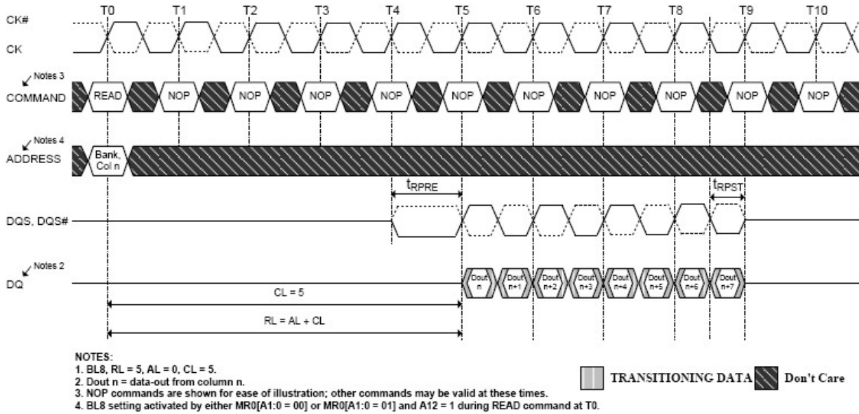
Figure 4-15 READ Burst Operation RL=5 (AL=0, CL=5, BL=8)
