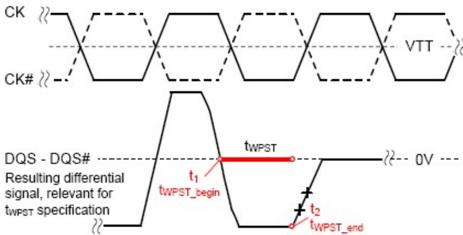
Figure 4-24 Method for calculating t WPST transitions and endpoints
