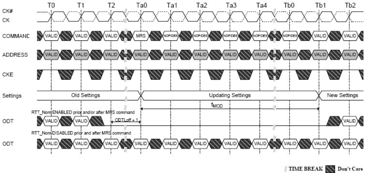
Figure 4-4 tMOD timing
