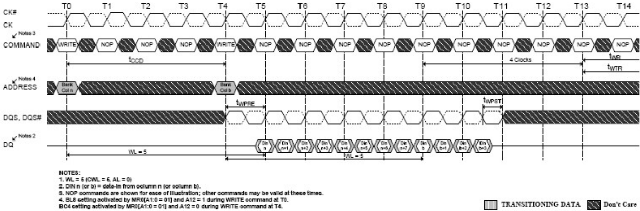
Figure 4-75 WRITE (BC8) to WRITE (BC4) OTF
