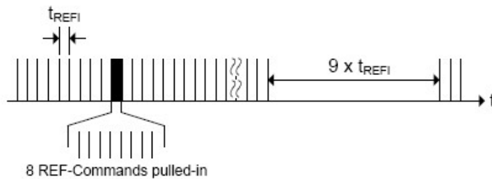
Figure 4-27 Pulling-in Refresh Commands (Example)
