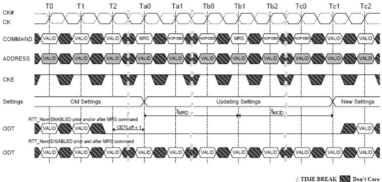
Figure 4-3 tMRD timing
