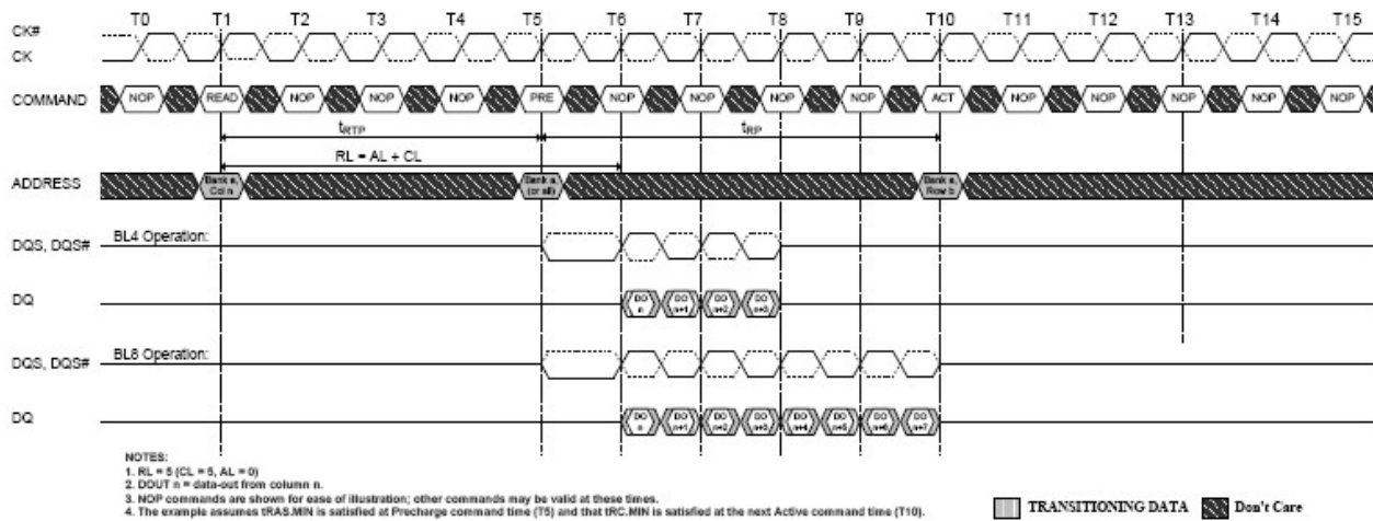
Figure 4-62 READ to PRECHARGE, RL = 5, AL = 0, CL = 5, tRTP = 4, tRP = 5
