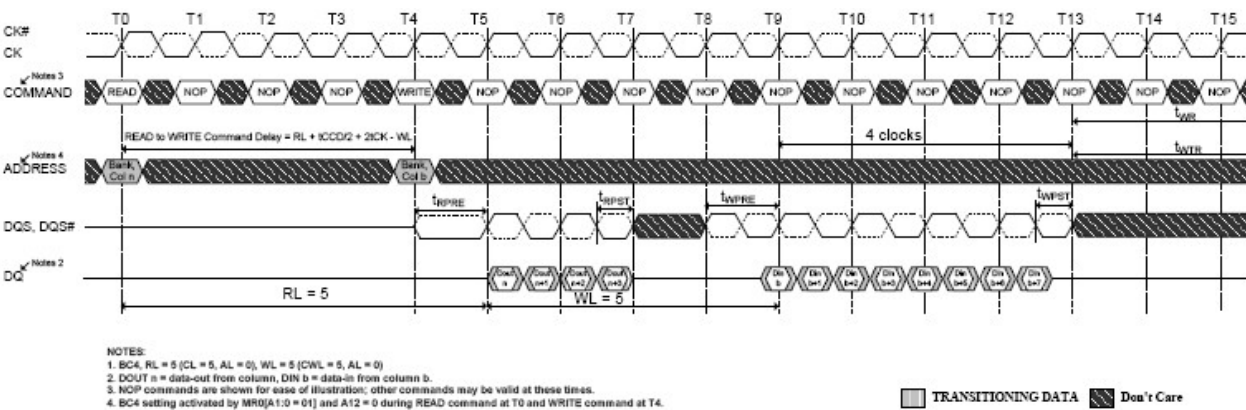
Figure 4-60 READ (BC4) to WRITE (BL8) OTF
