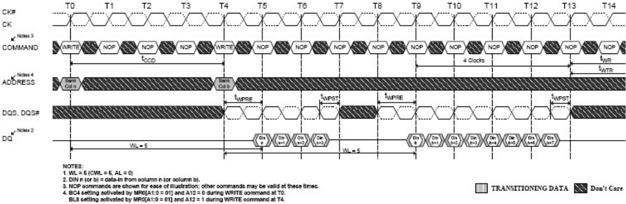
Figure 4-76 WRITE (BC4) to WRITE (BC8) OTF
