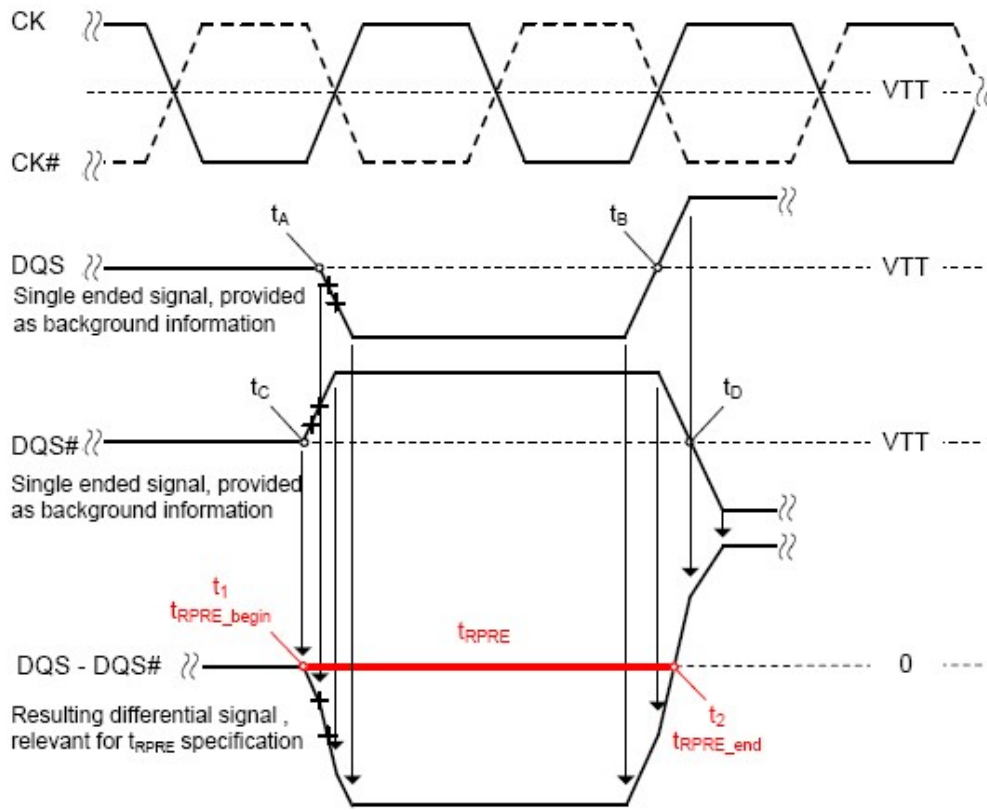
Figure 4-21 Method for calculating t RPRE transitions and endpoints
