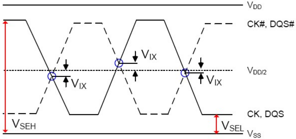
Figure 4-32 Vix Definition
