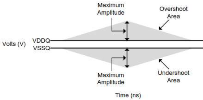
Figure 4-39 Clock, Data, Strobe and Mask Overshoot and Undershoot Definition
