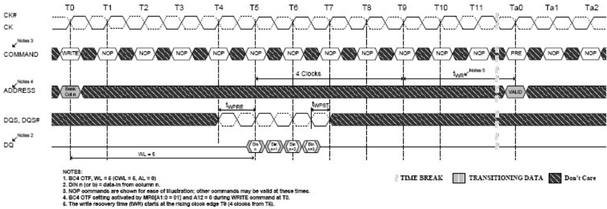
Figure 4-69 WRITE (BC4) OTF to precharge operation
