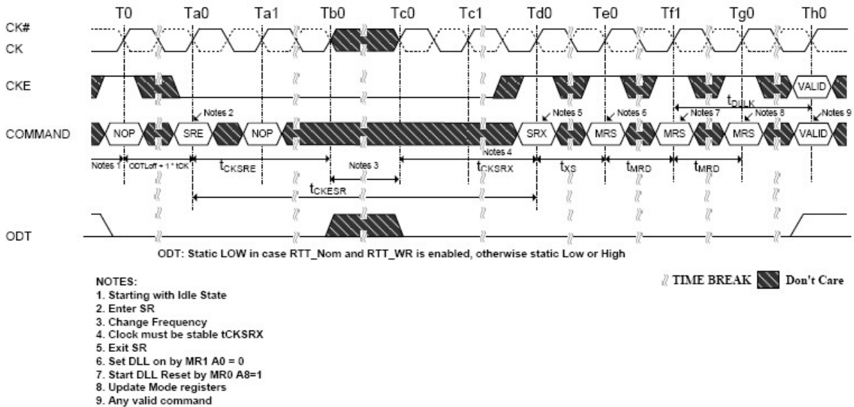
Figure 4-10 DLL Switch Sequence from DLL-off to DLL on
